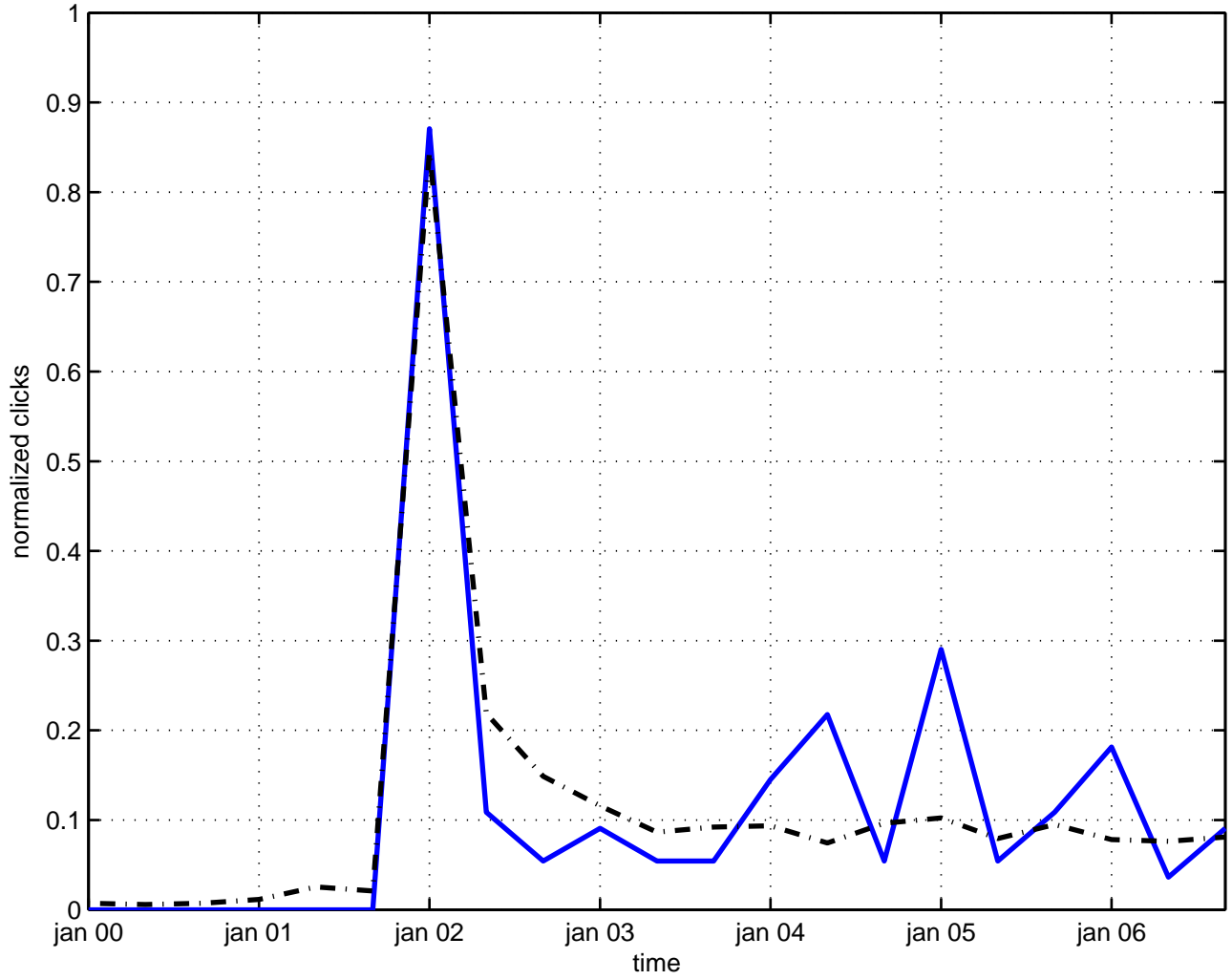
o(n,m) symmetry
