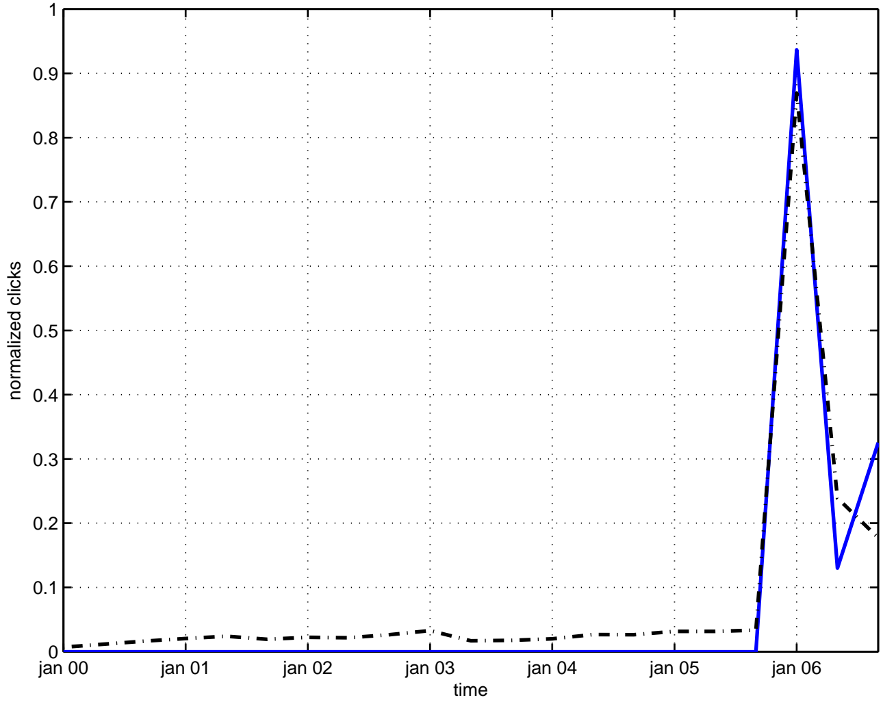
o(n,1) group theory
