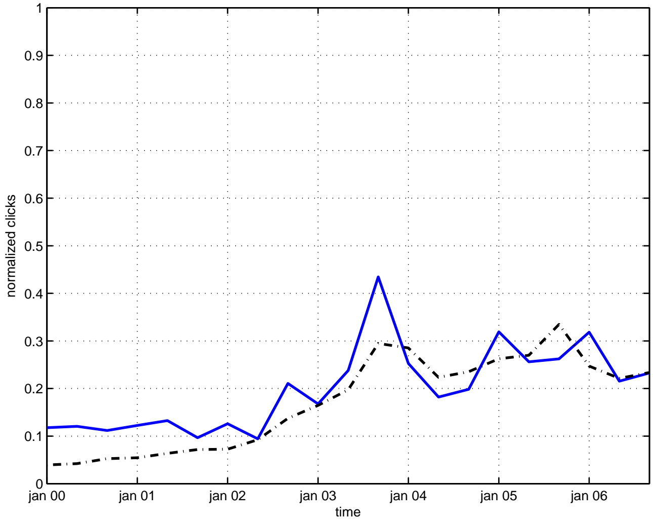
o(n) symmetry
