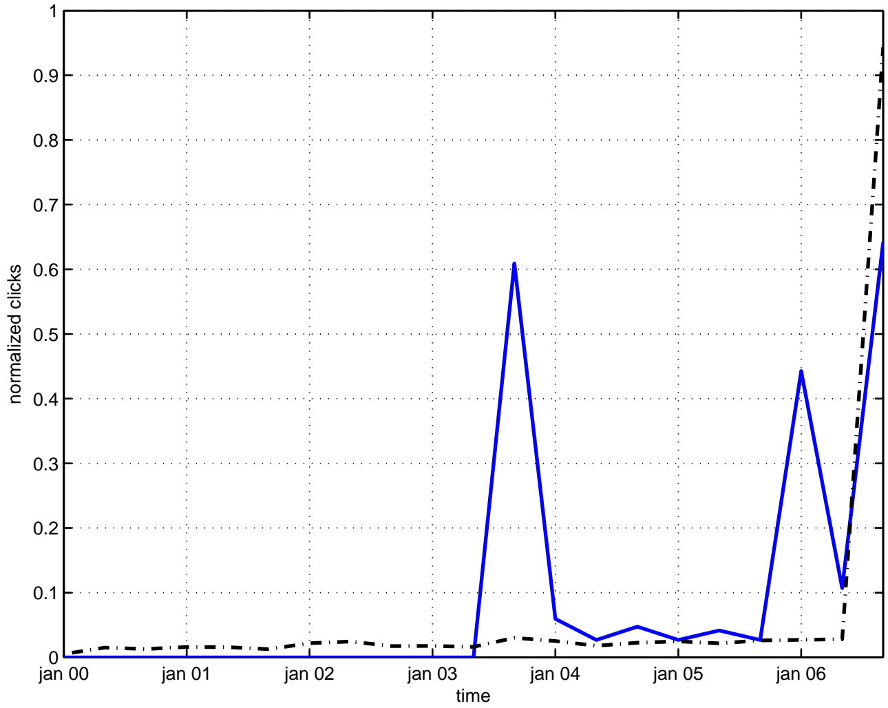
o(n) gauge field theory
