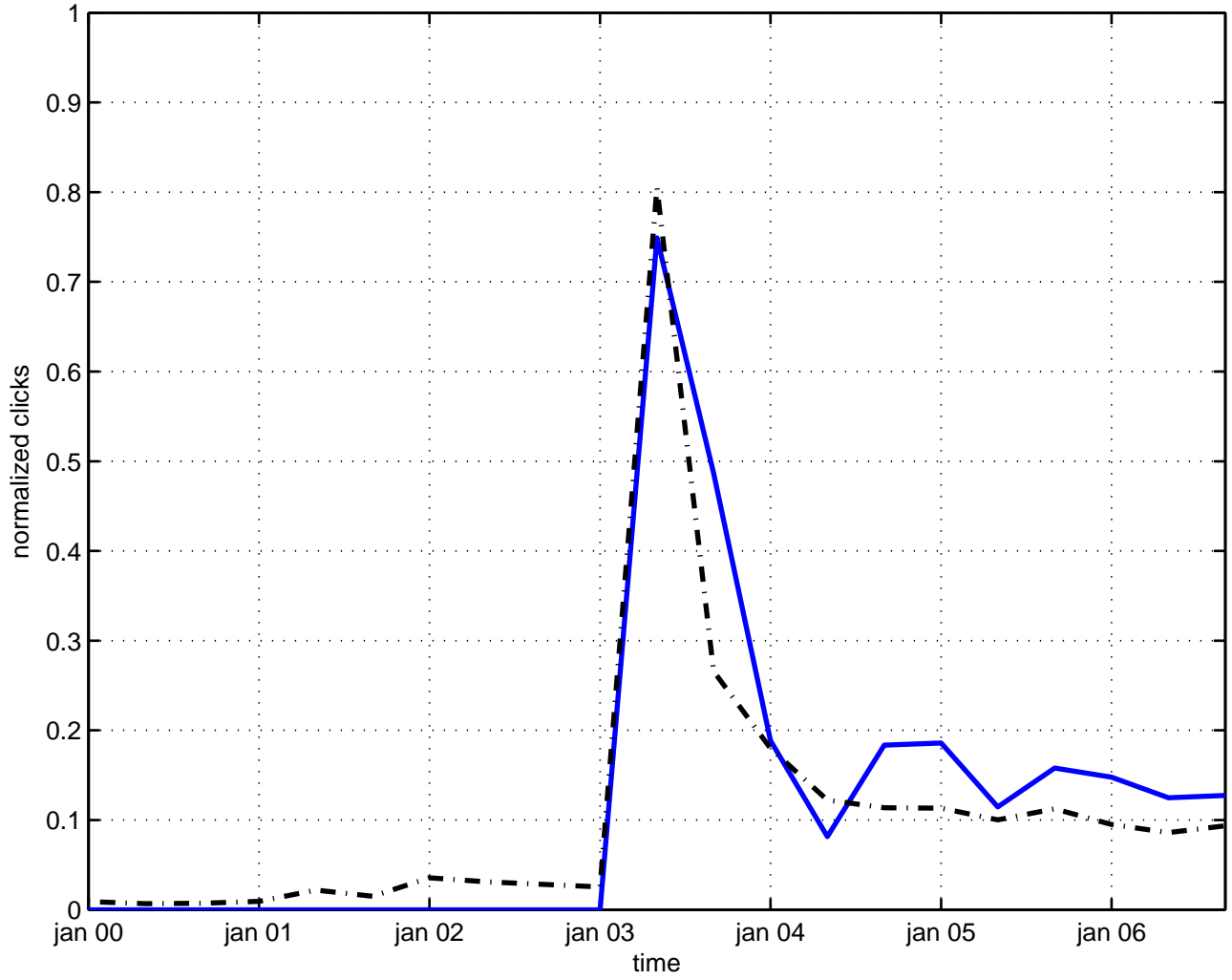
o(6) sigma model
