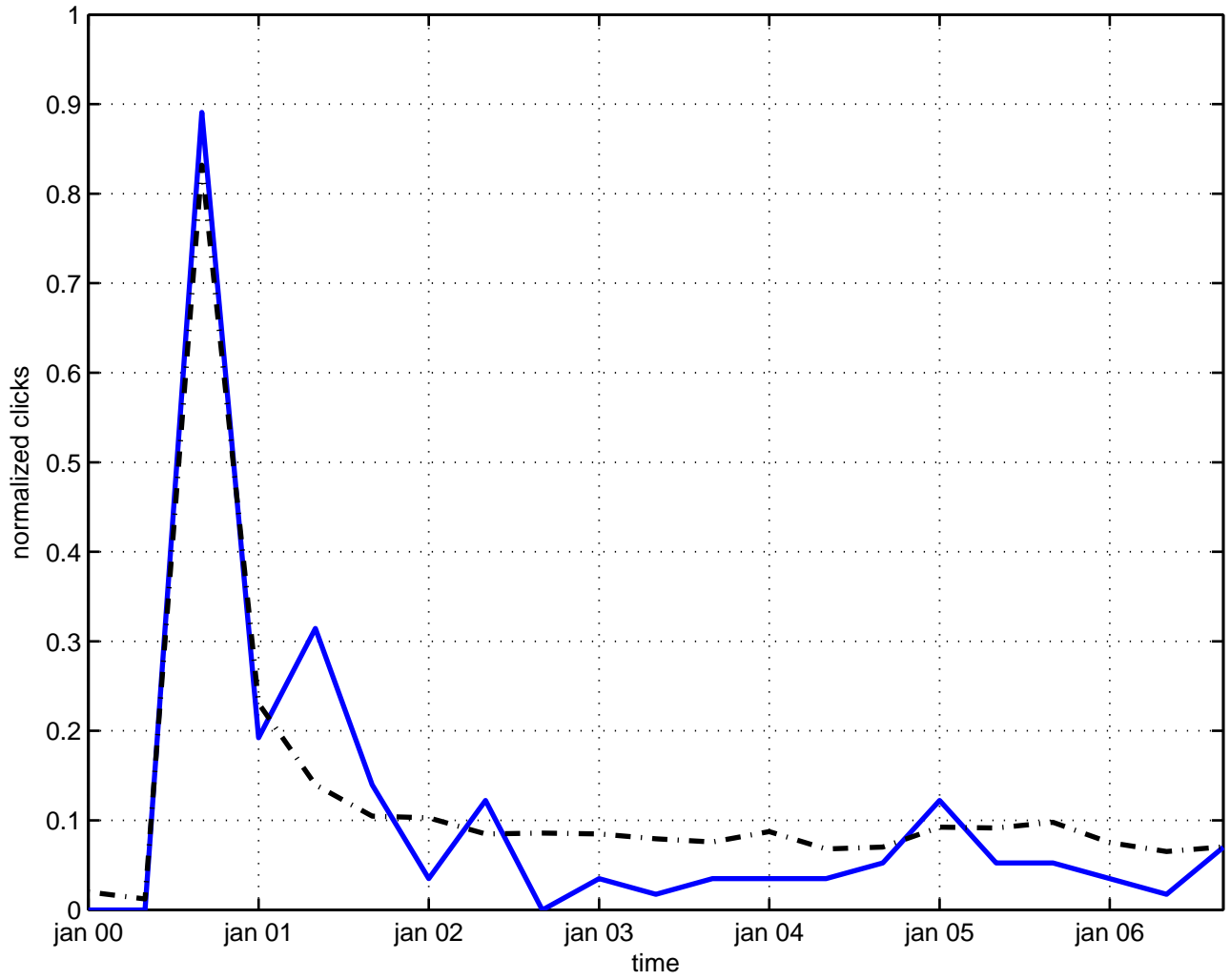
o(5) gauge field theory
