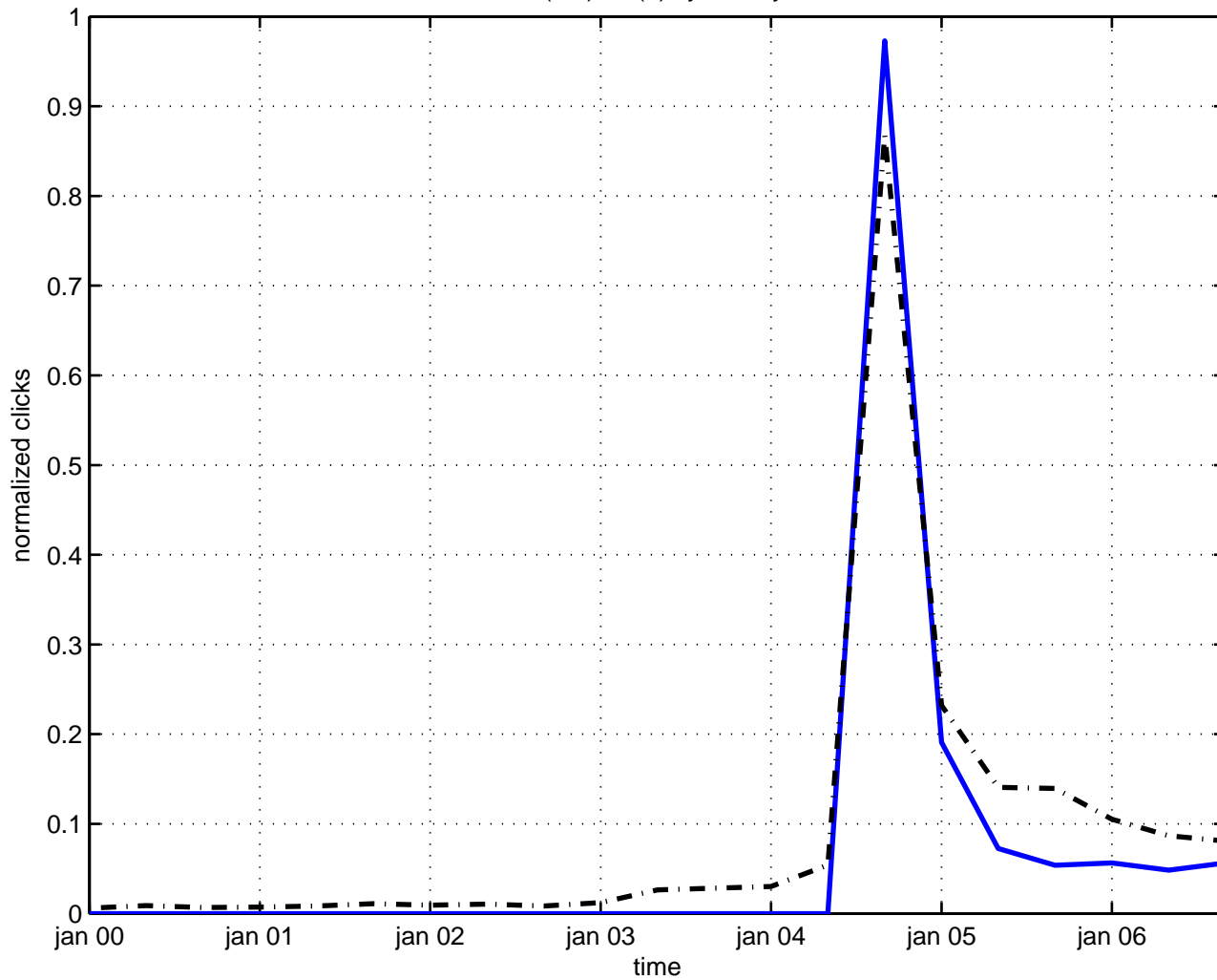
o(4,2) \times o(6) symmetry
