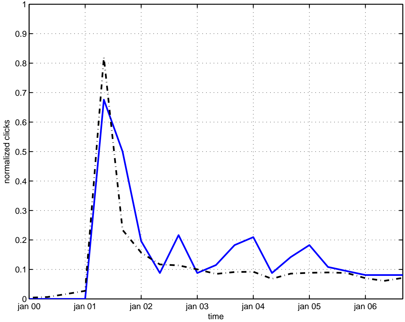
o(4,2) symmetry
