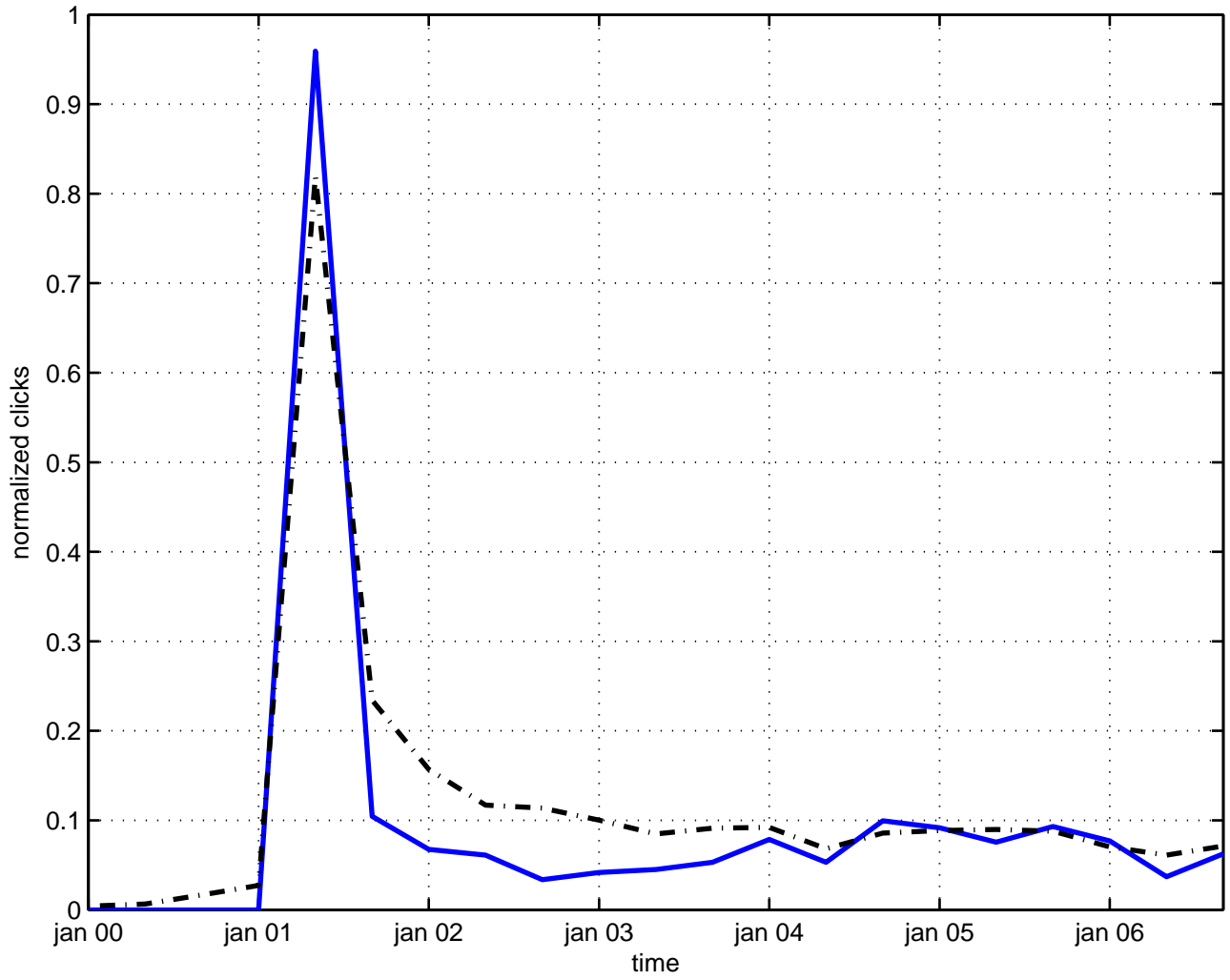
o(4) group theory
