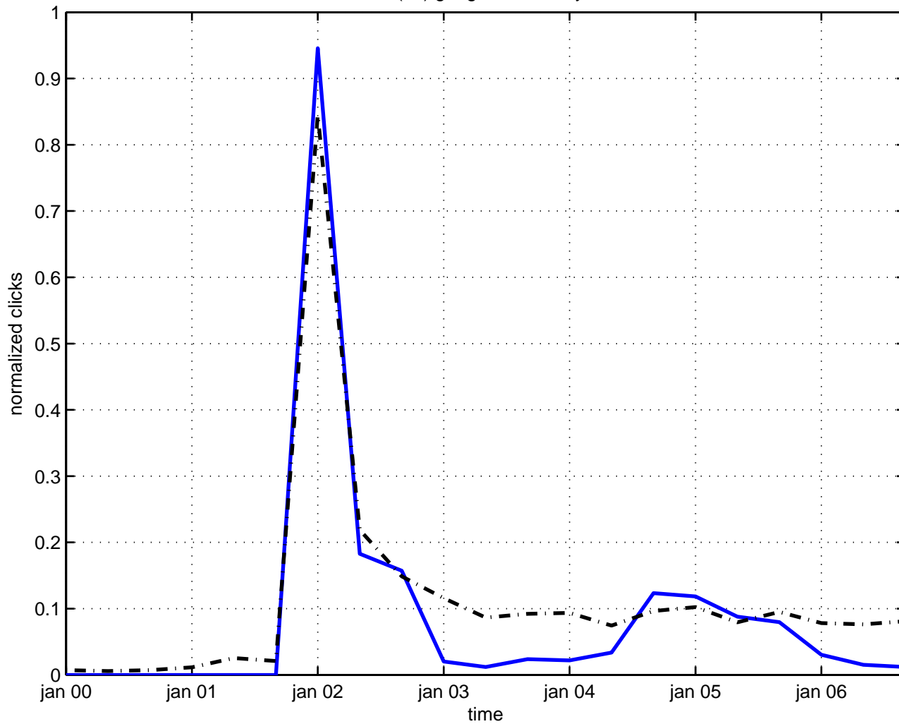
o(32) gauge field theory
