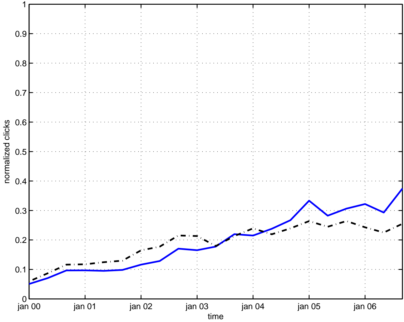
numerical calculations
