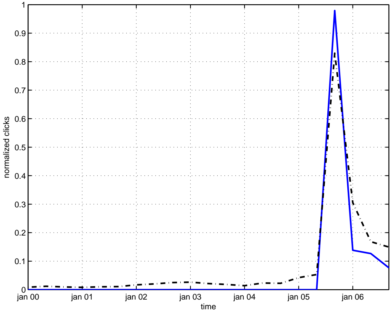
nucleon
