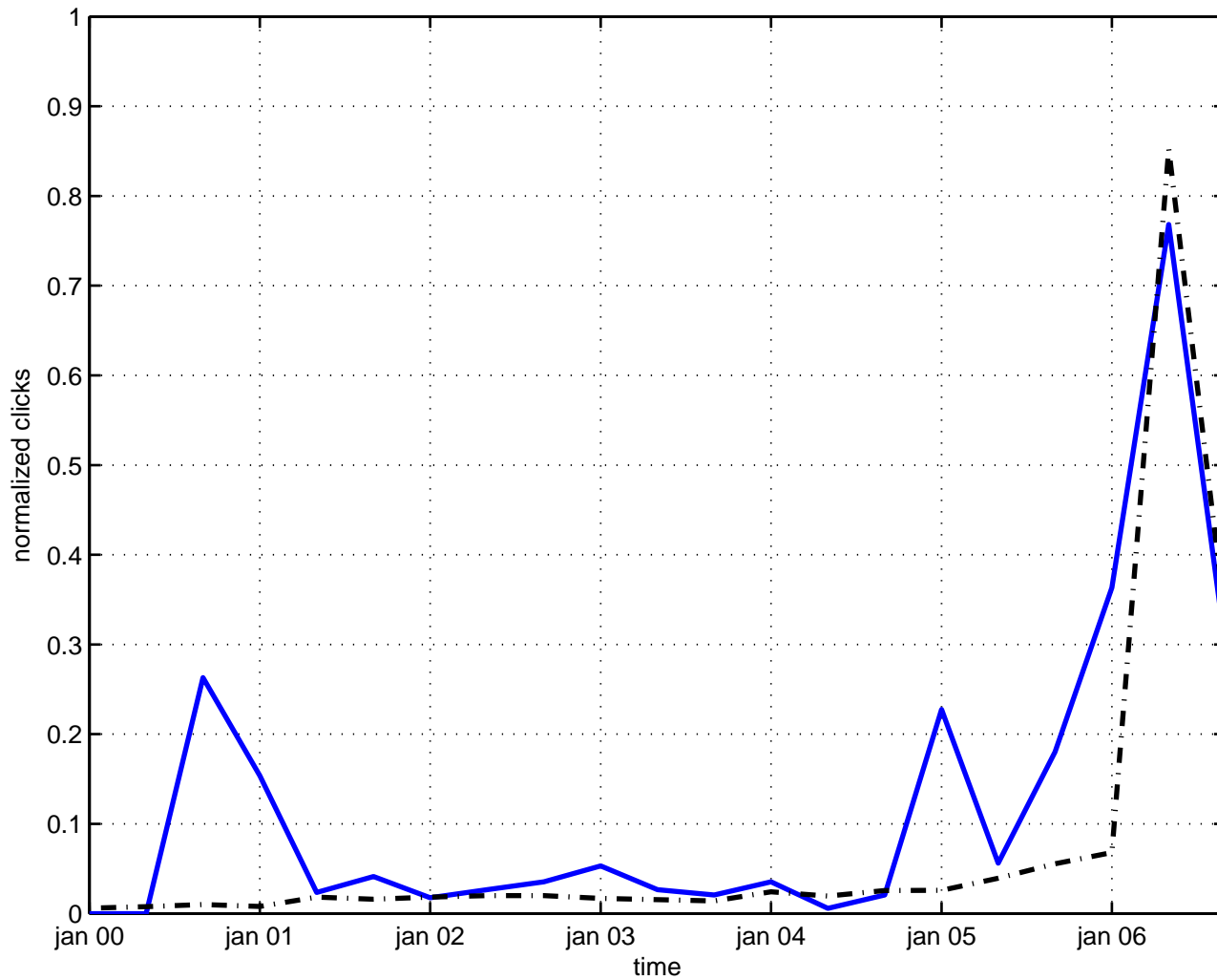
nuclear model
