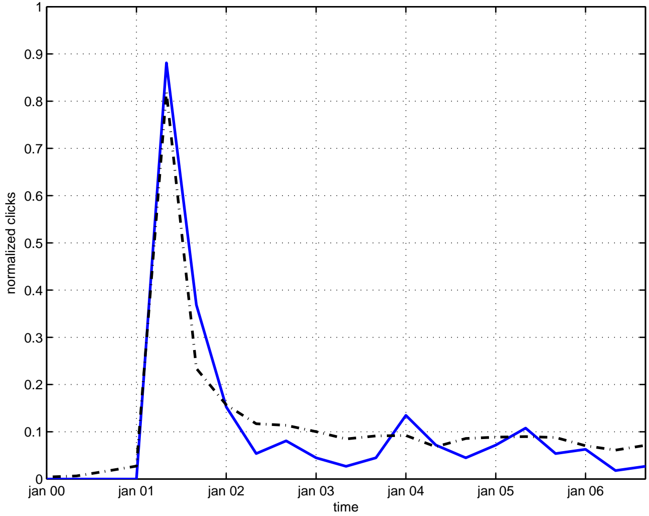
nonrenormalizable field theory
