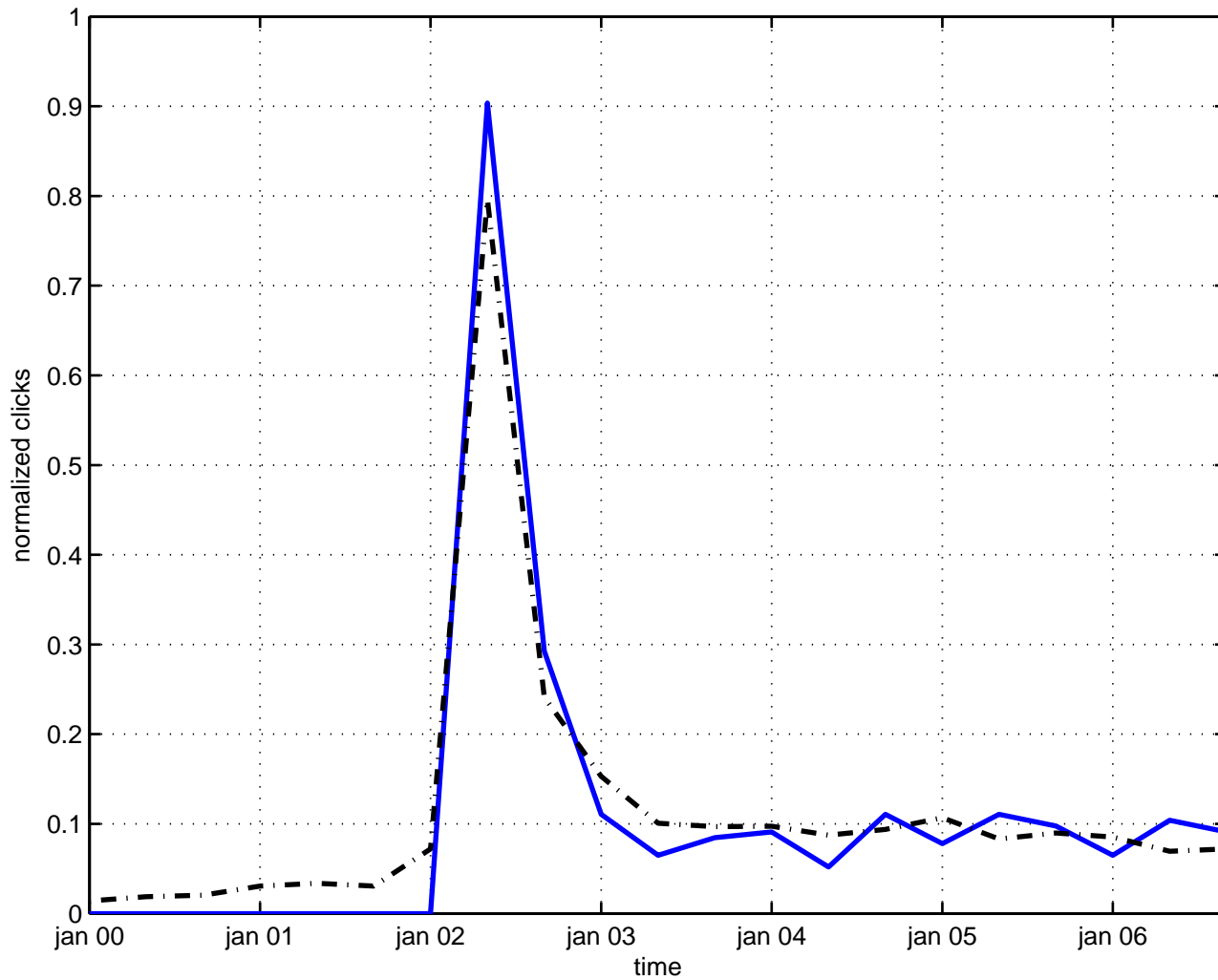
nonrelativistic s-matrix
