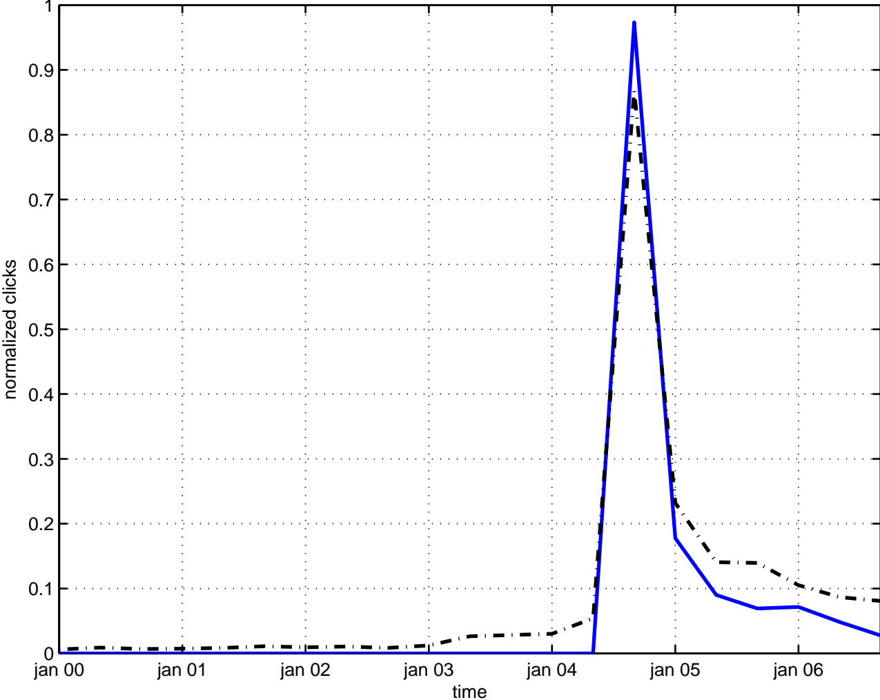
nonrelativistic neutrino
