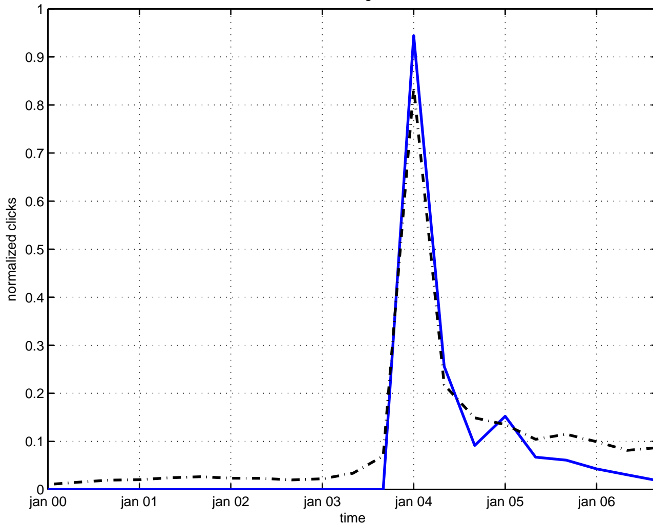
nonrelativistic gravitation
