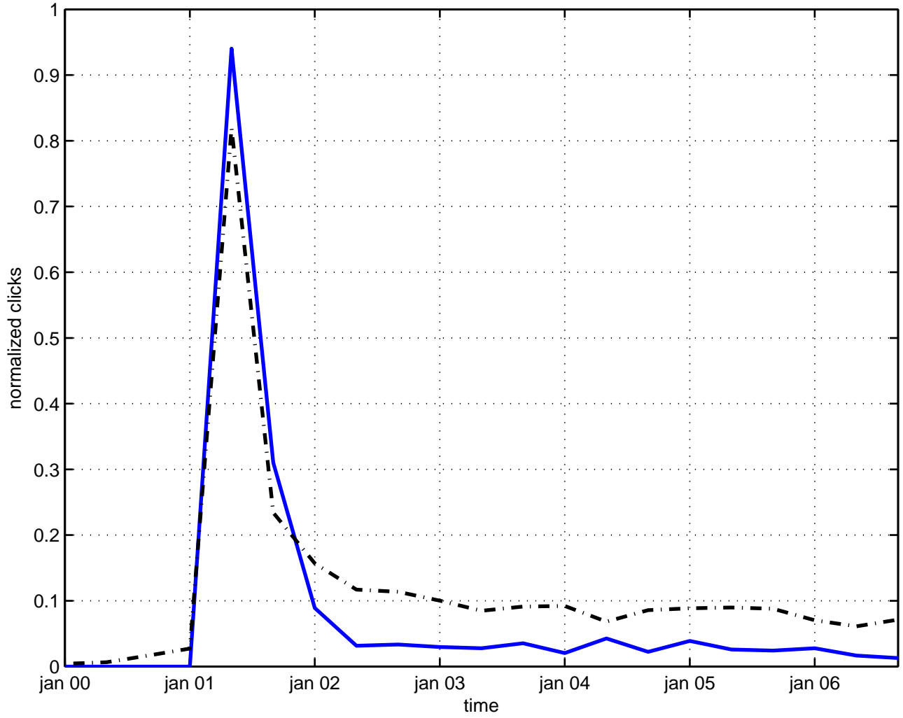
nonpolynomial field theory
