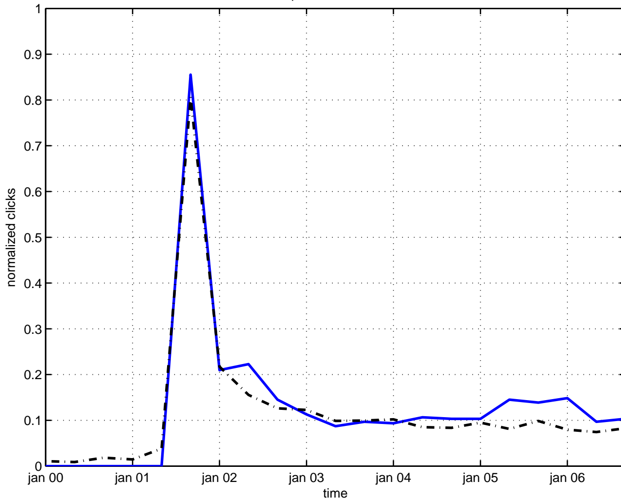
nonperturbative soliton
