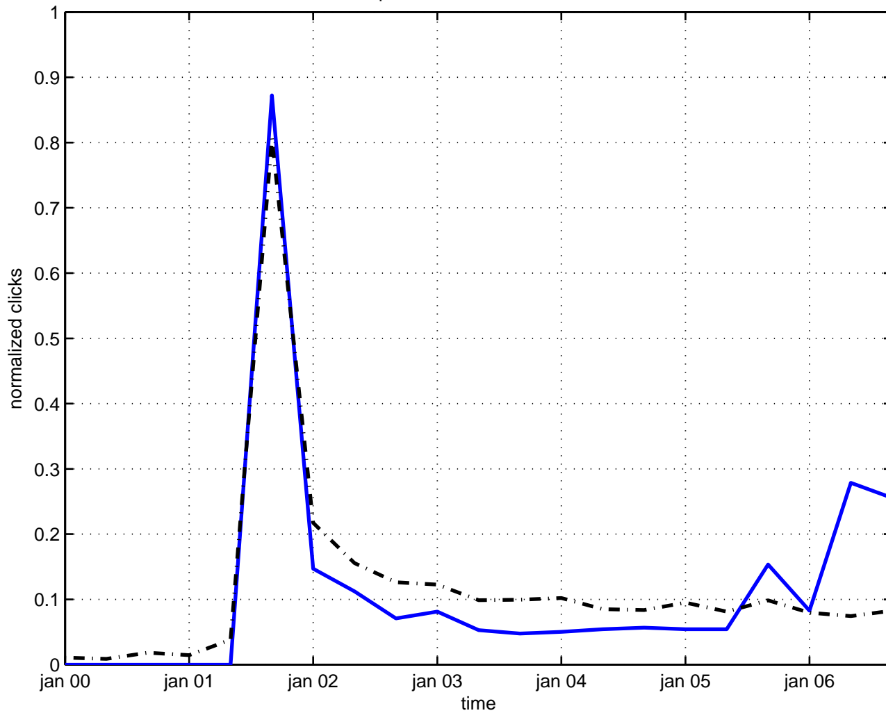
nonperturbative renormalization
