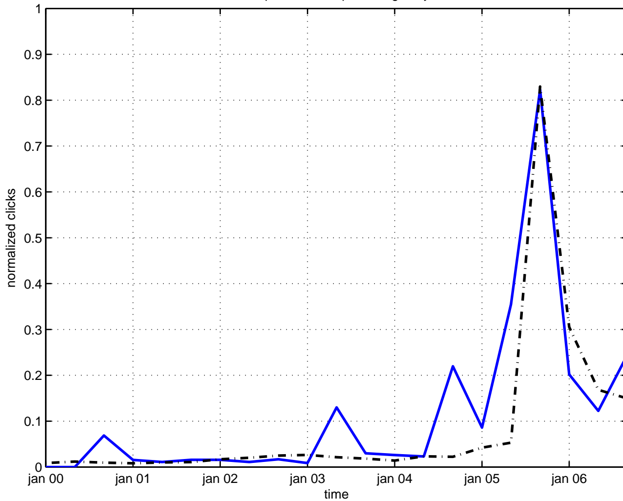
nonperturbative quantum gravity
