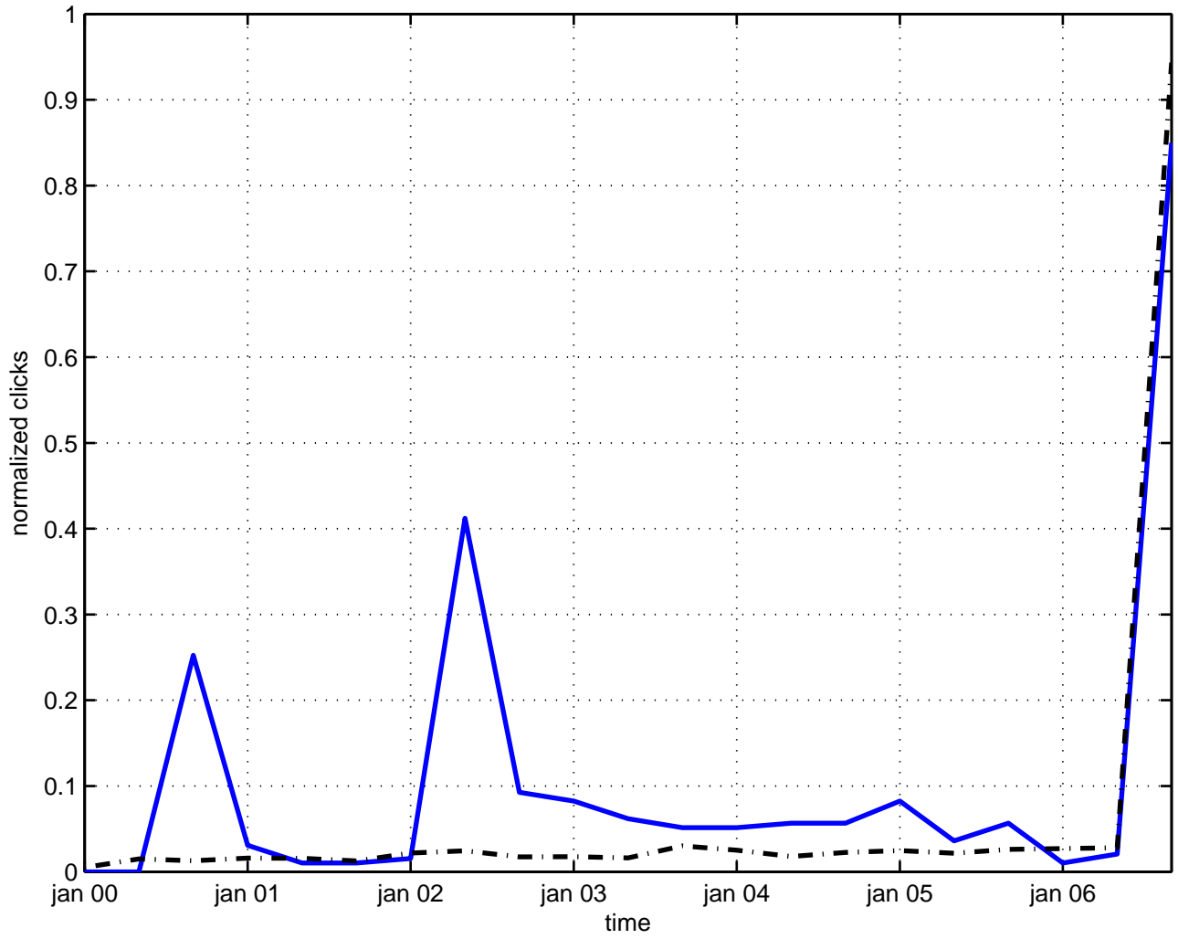
nonperturbative quantization
