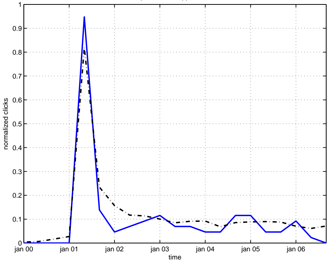
nonperturbative approximation
