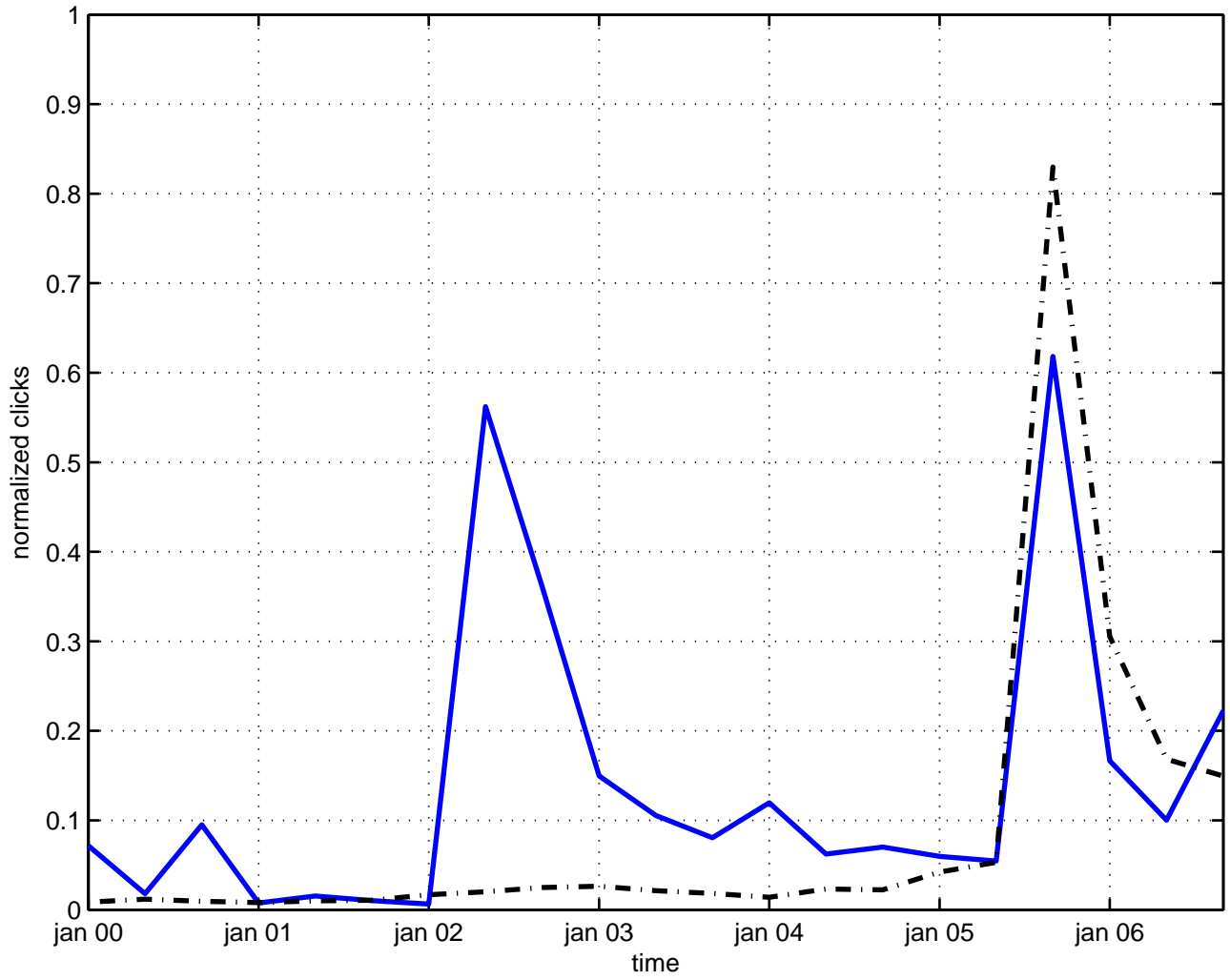
nonlocal transformation
