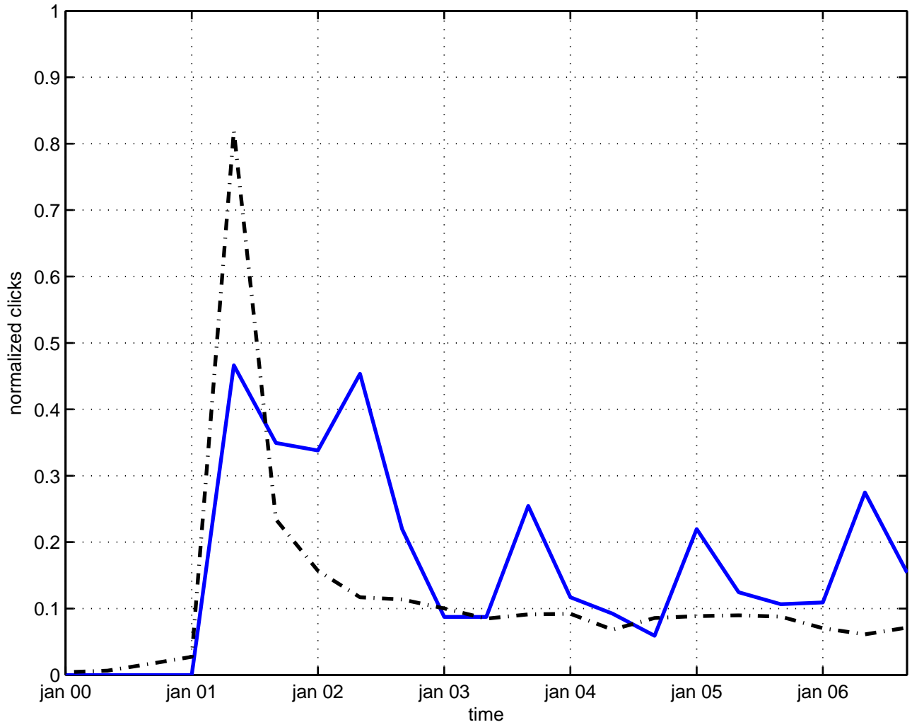
nonlocal string model
