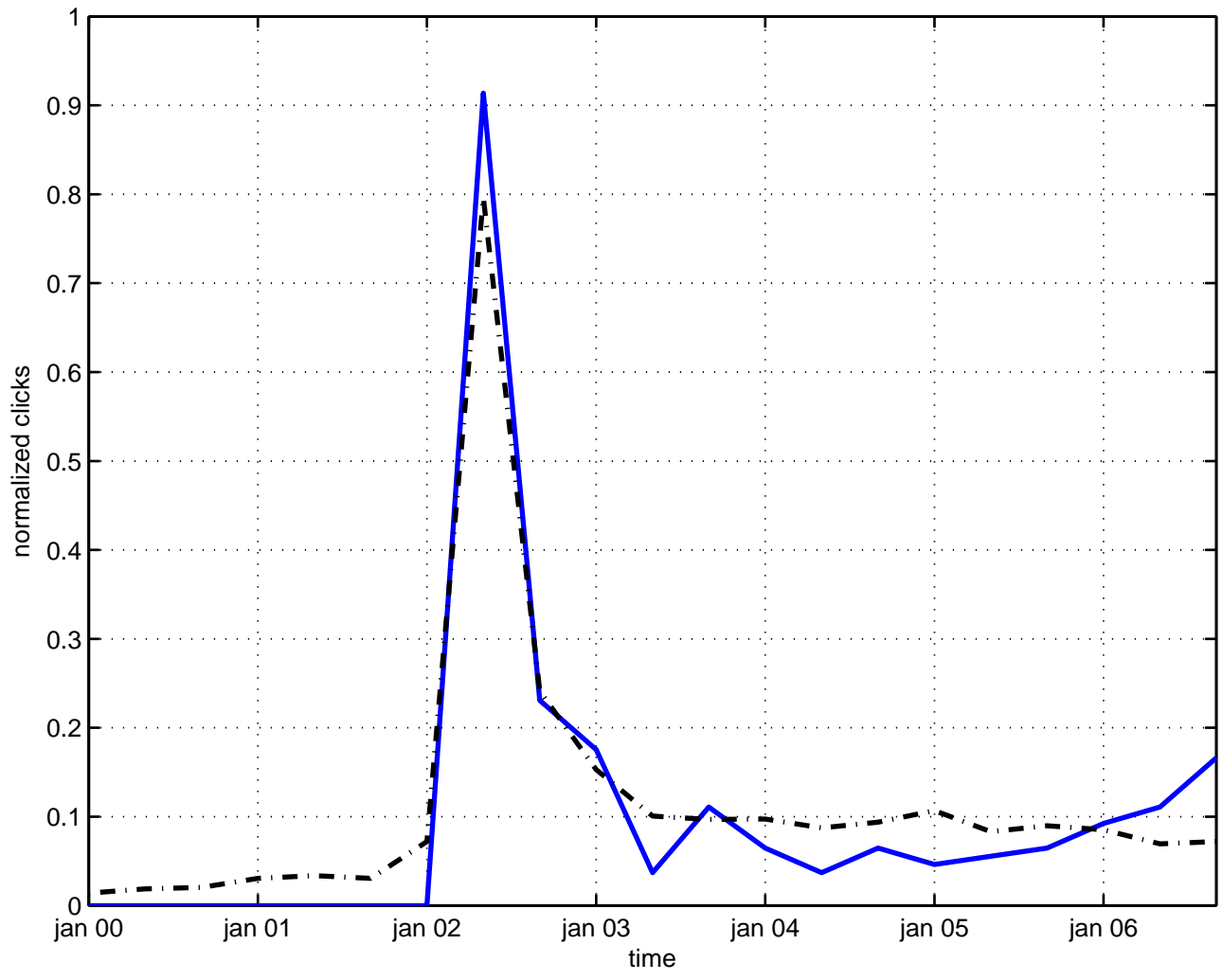
nonlocal oscillator
