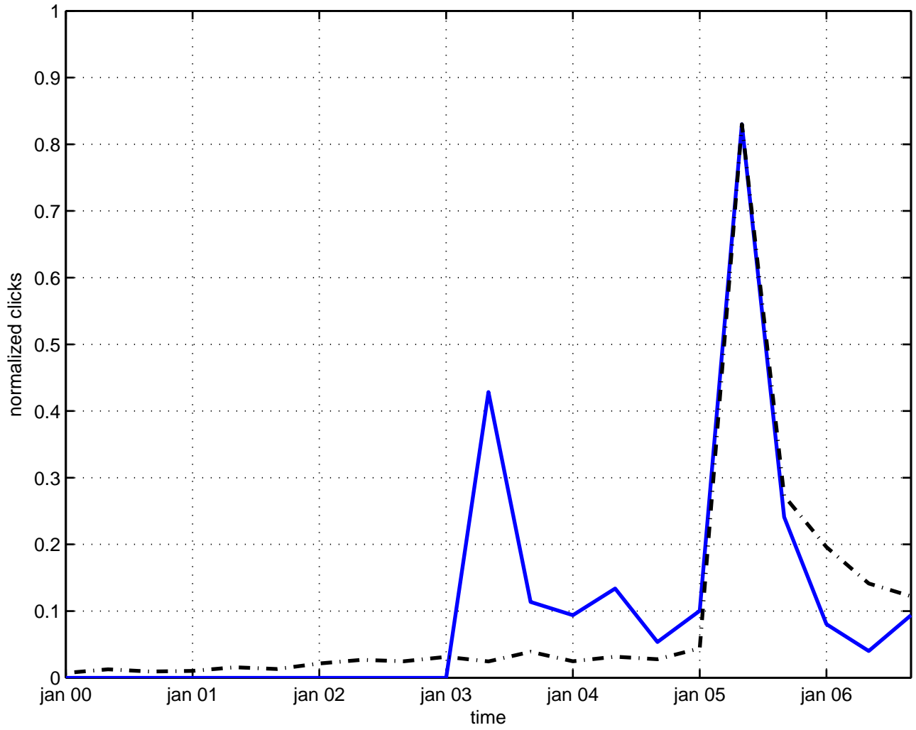
nonlocal mass
