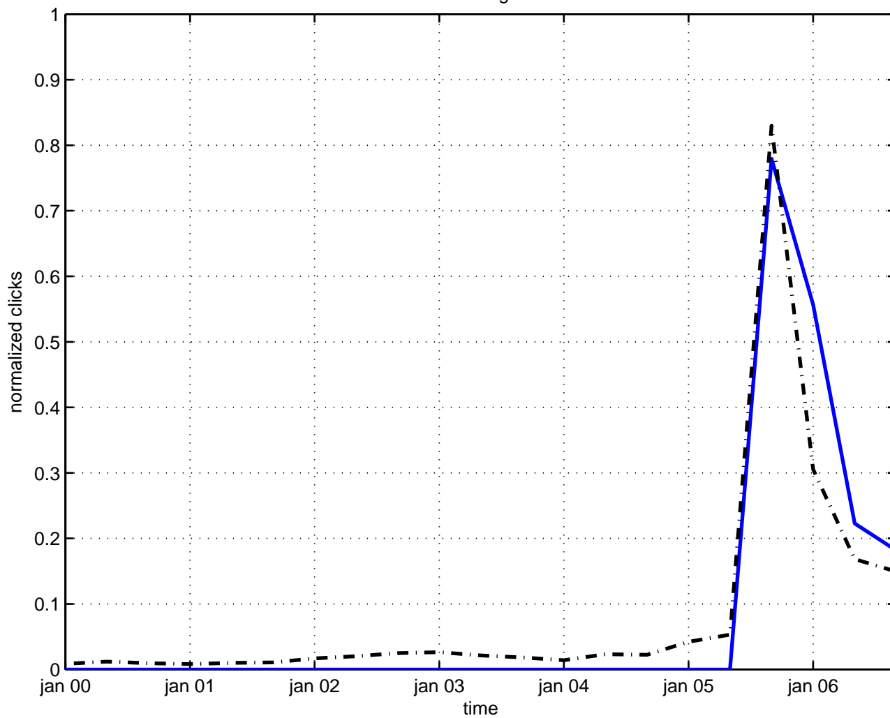
nonlocal ising model
