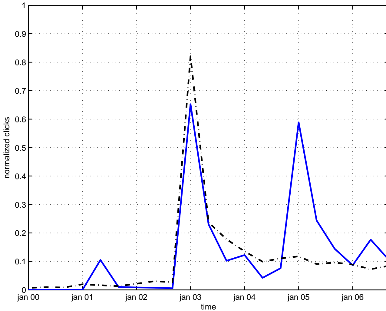
nonlocal interaction
