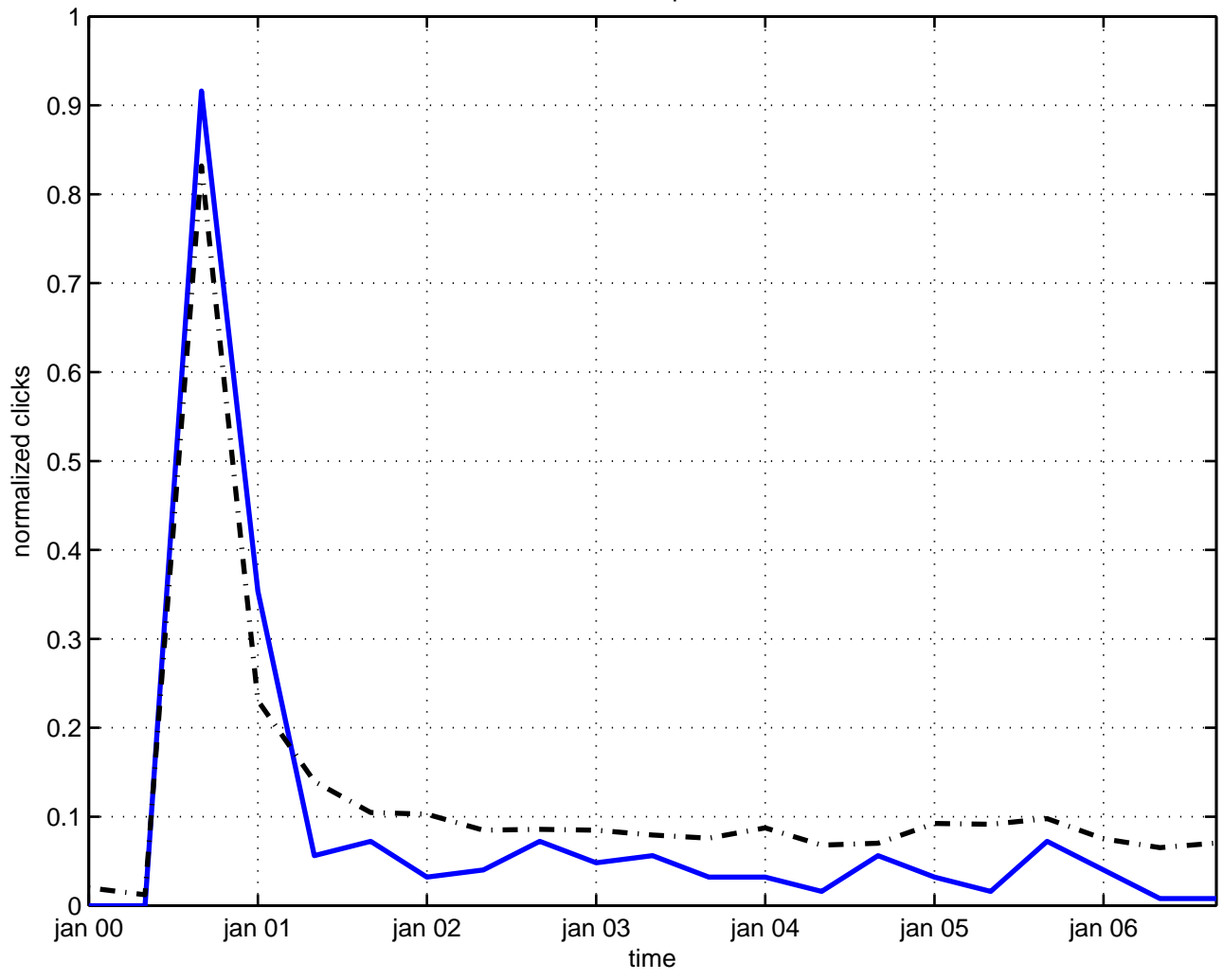
nonlocal expansion
