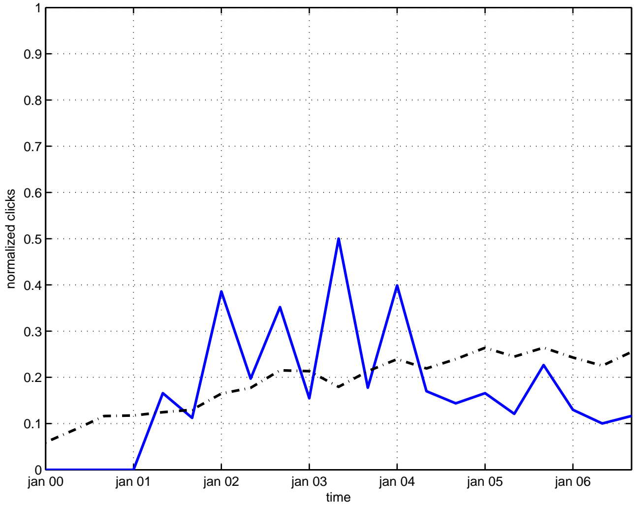
nonlocal effective action
