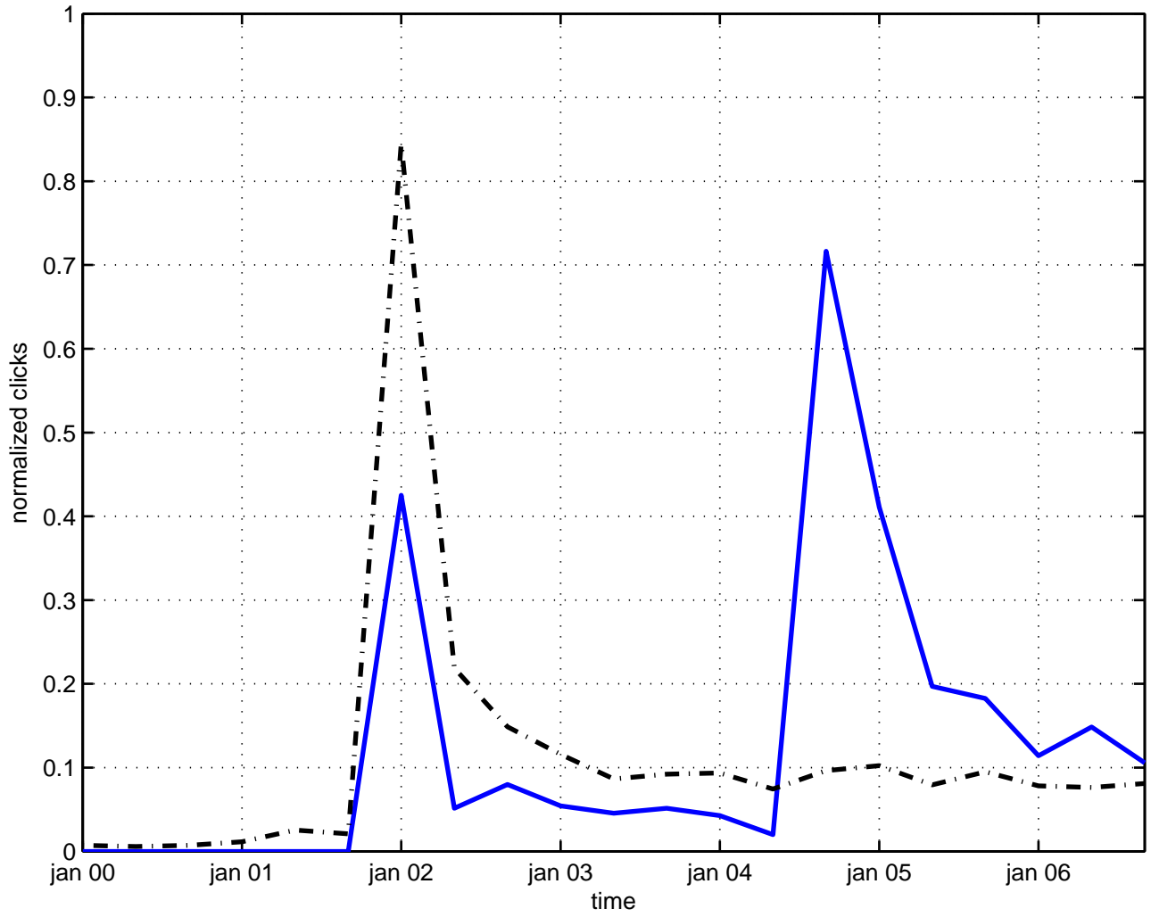
nonlocal current
