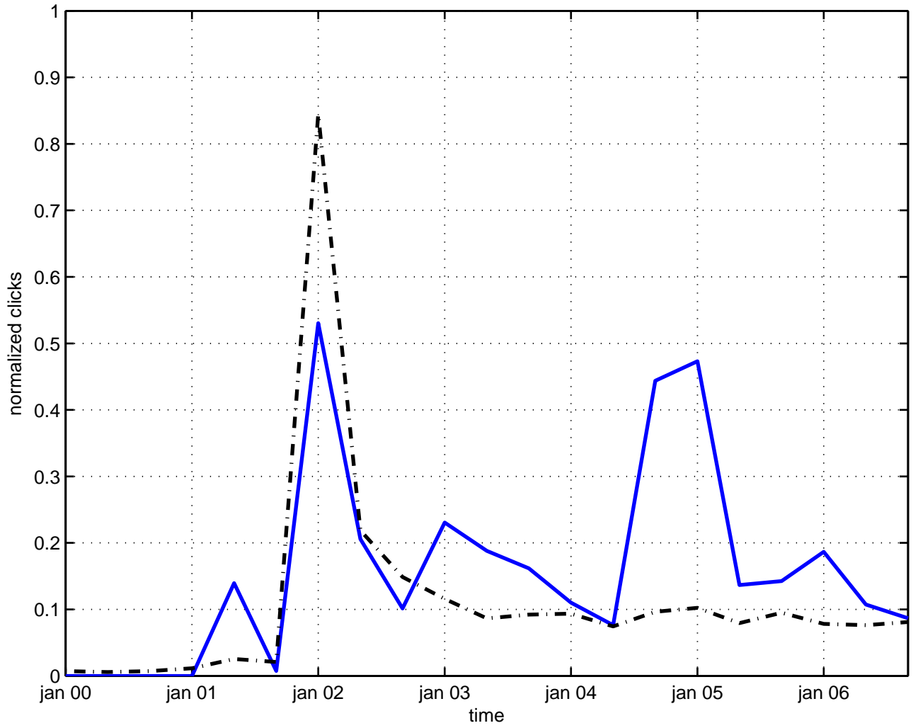
nonlocal action
