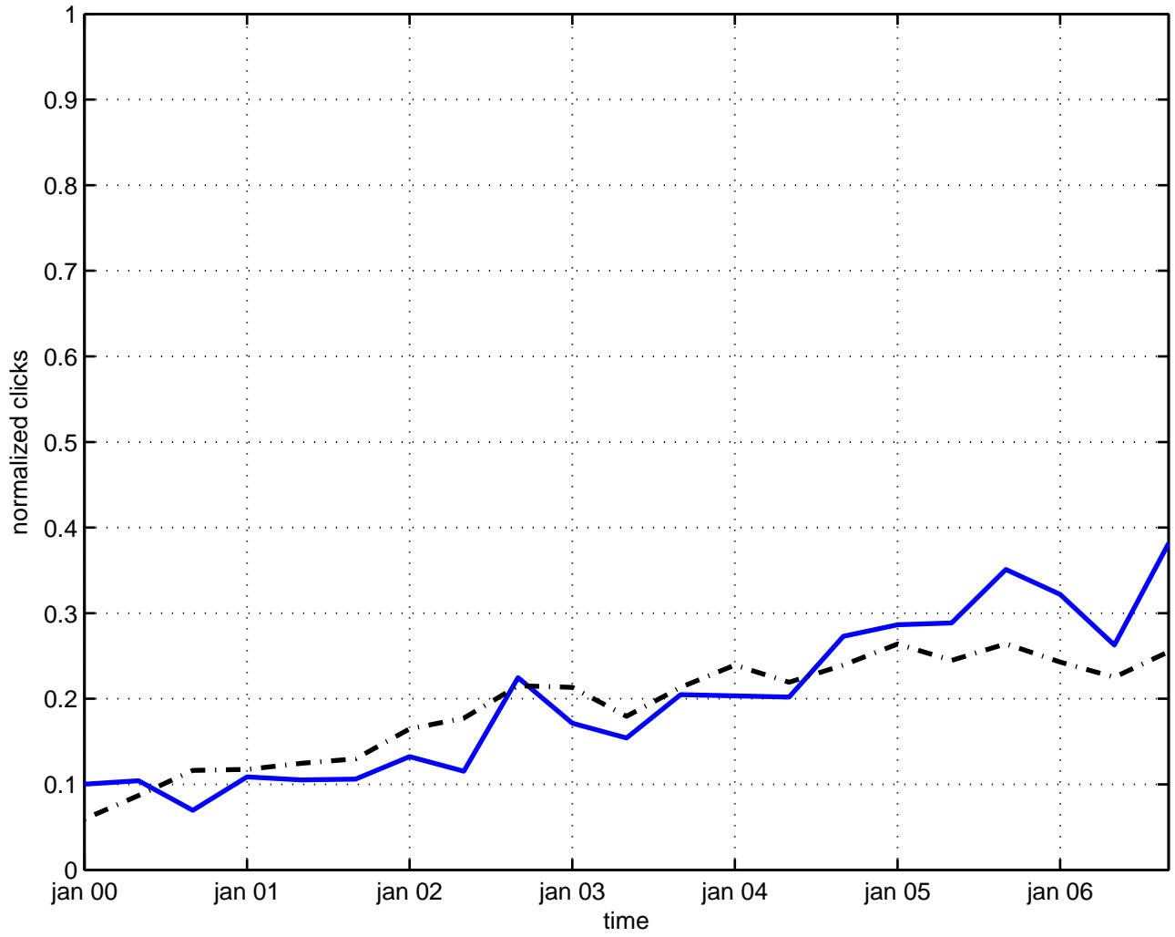
nonlinear sigma model
