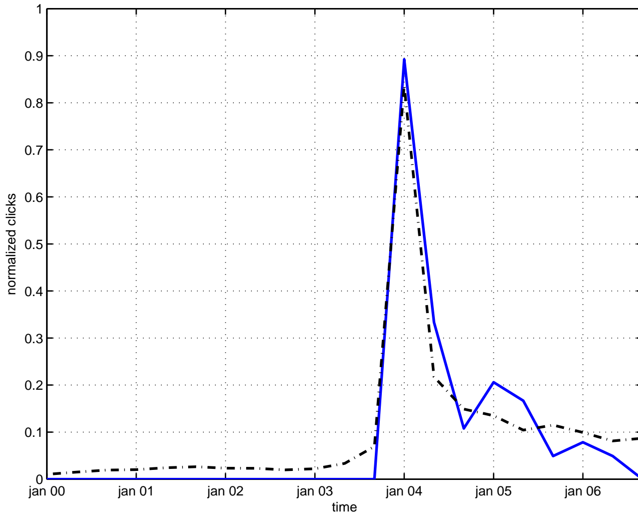
nonlinear radion
