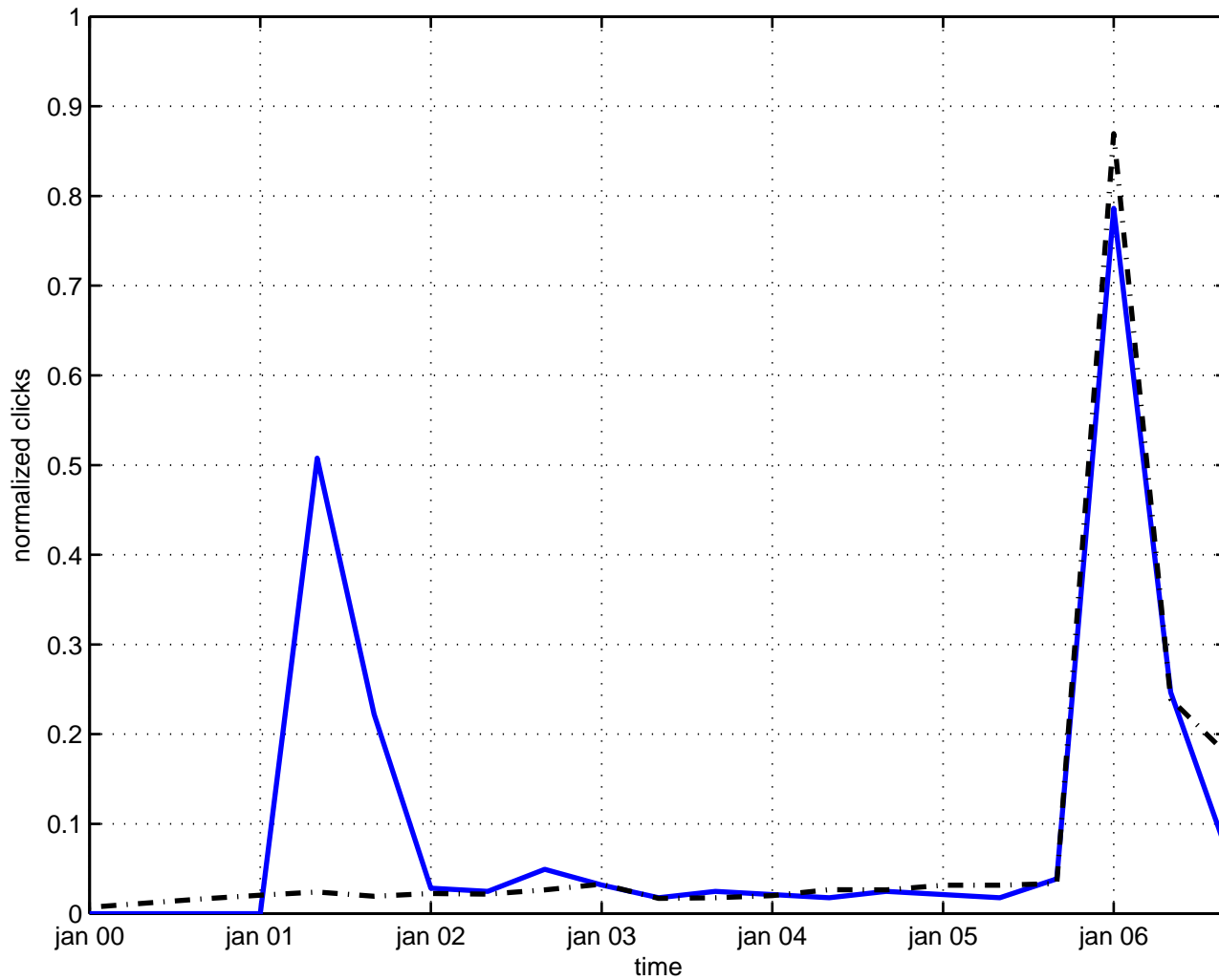
nonlinear oscillator
