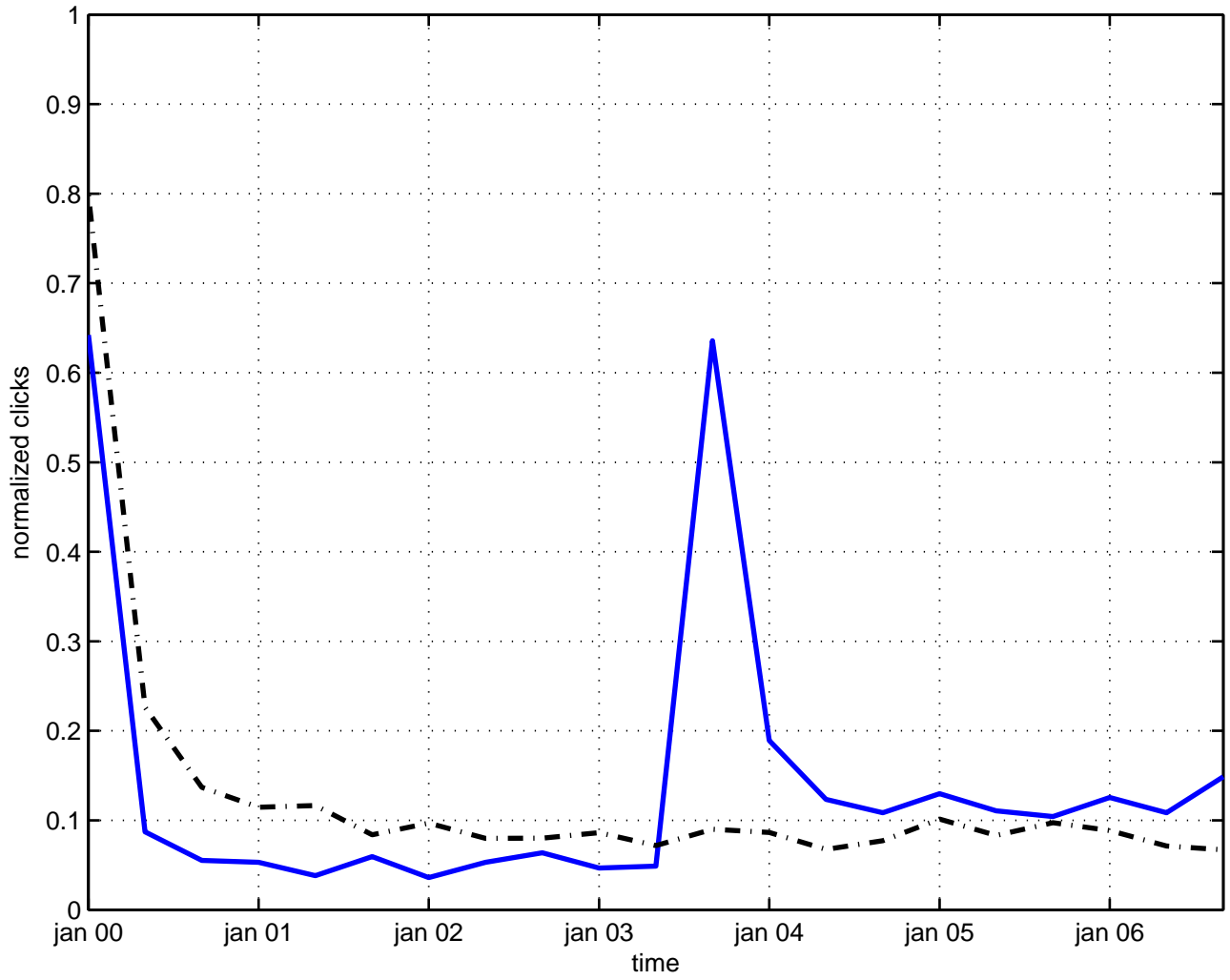
nonlinear optics
