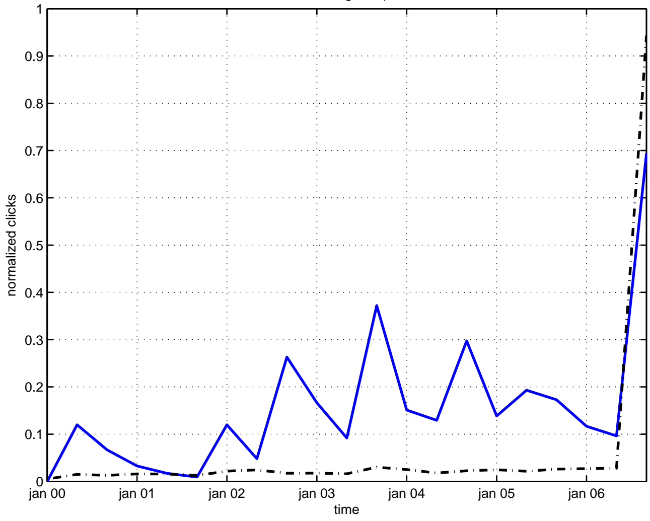
nonlinear integral equations
