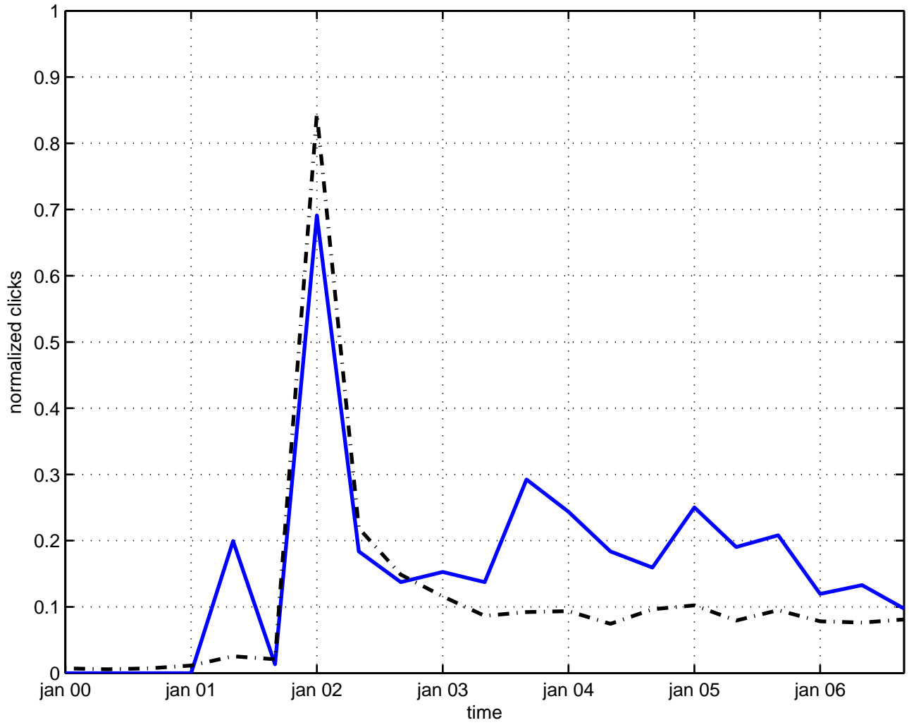
nonlinear instanton
