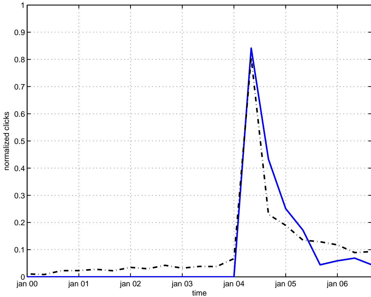
nonlinear hamiltonian formalism
