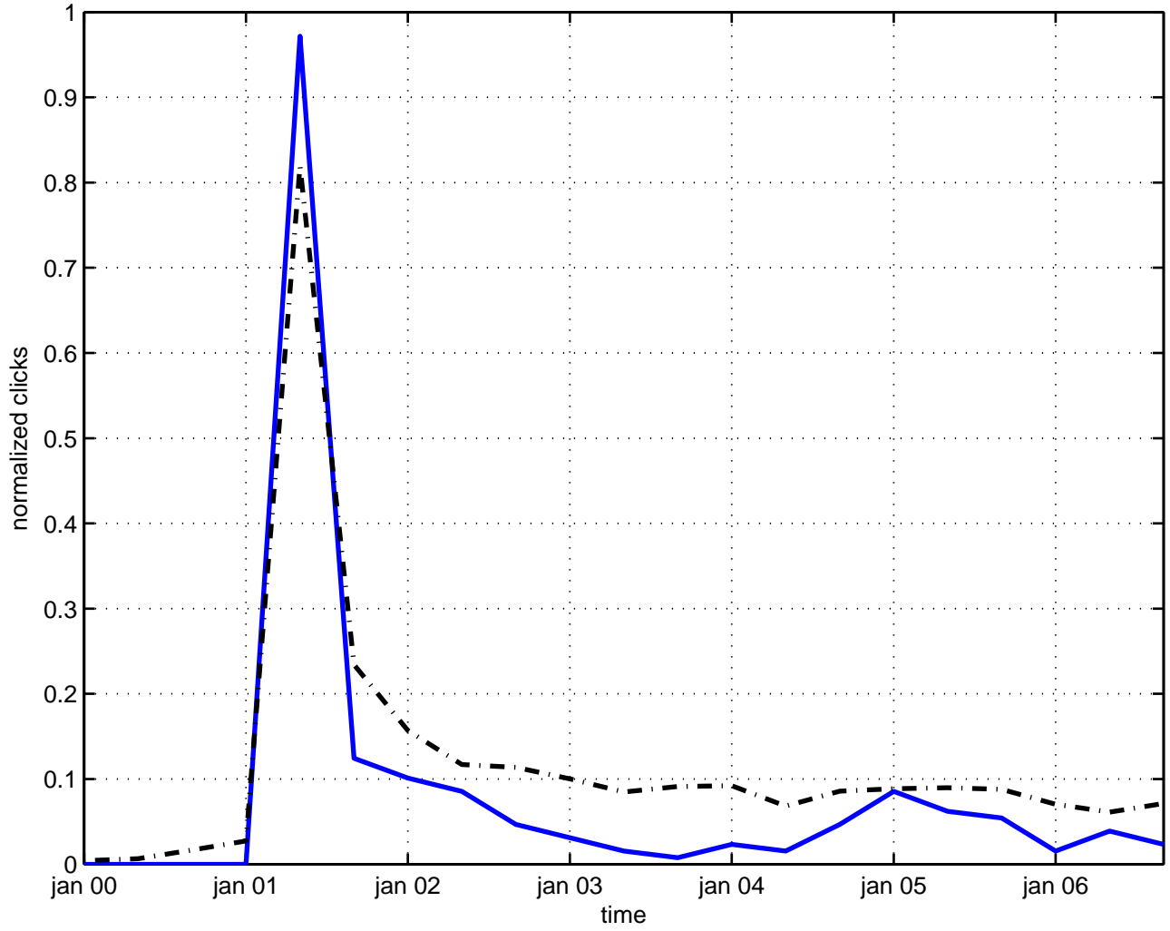
nonlinear fluctuation
