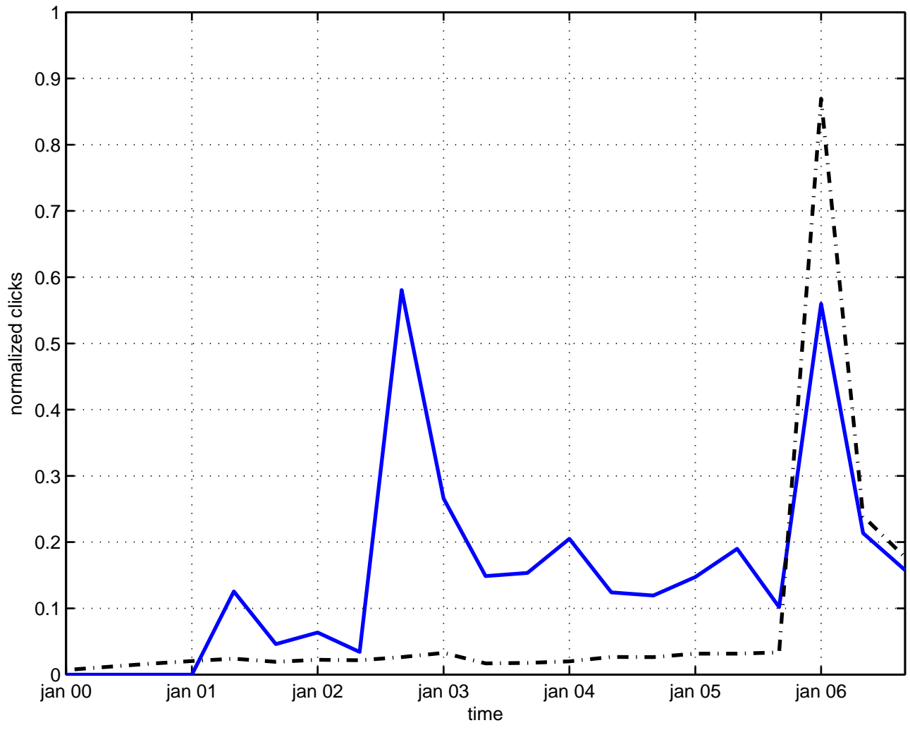
nonlinear effect
