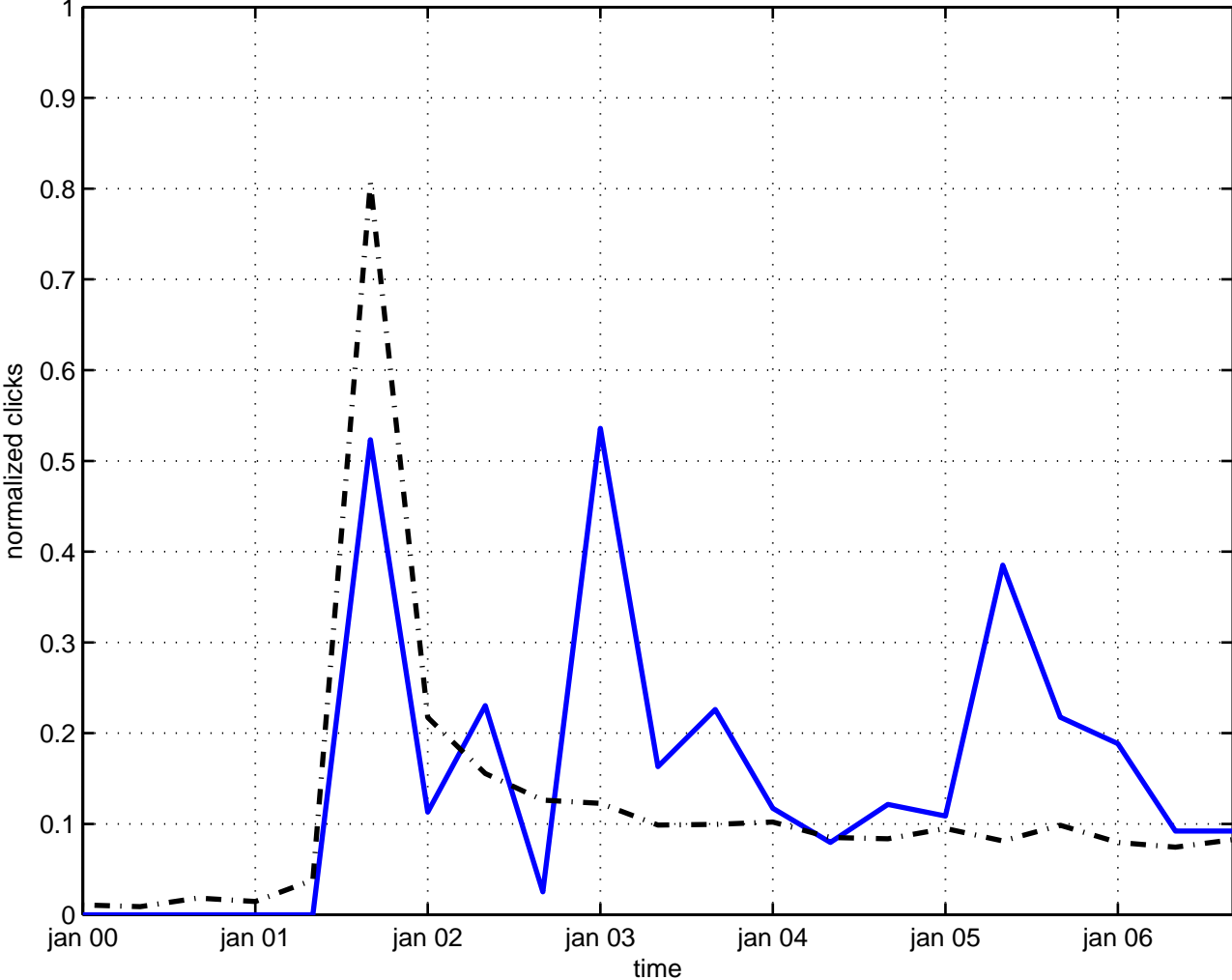
nonlinear constraint
