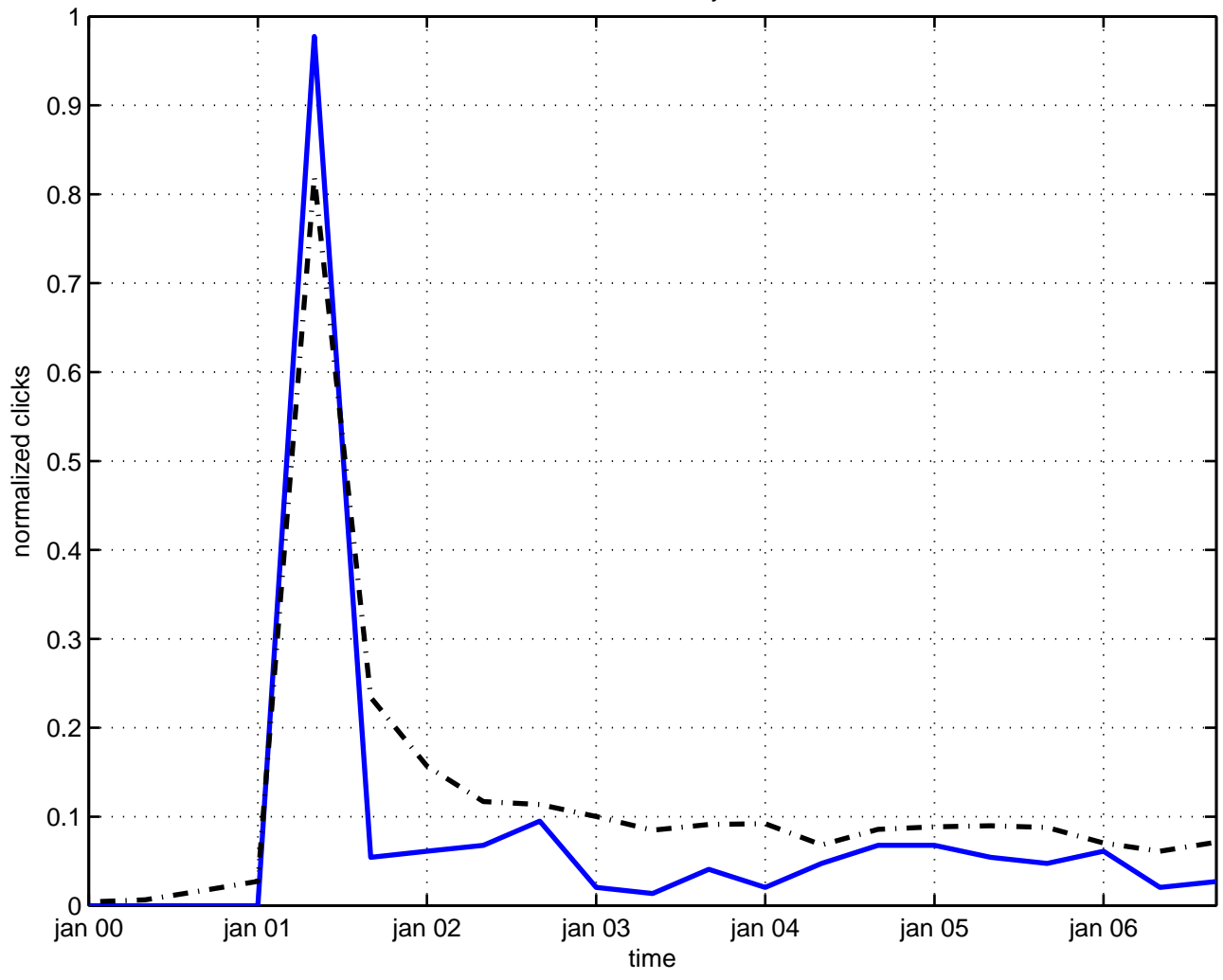
noncommutative xy model
