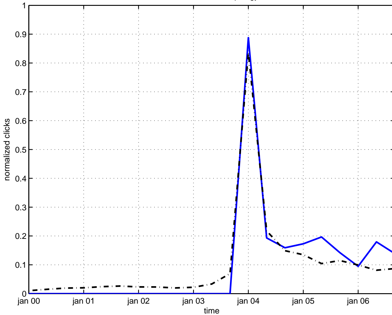
noncommutative topology
