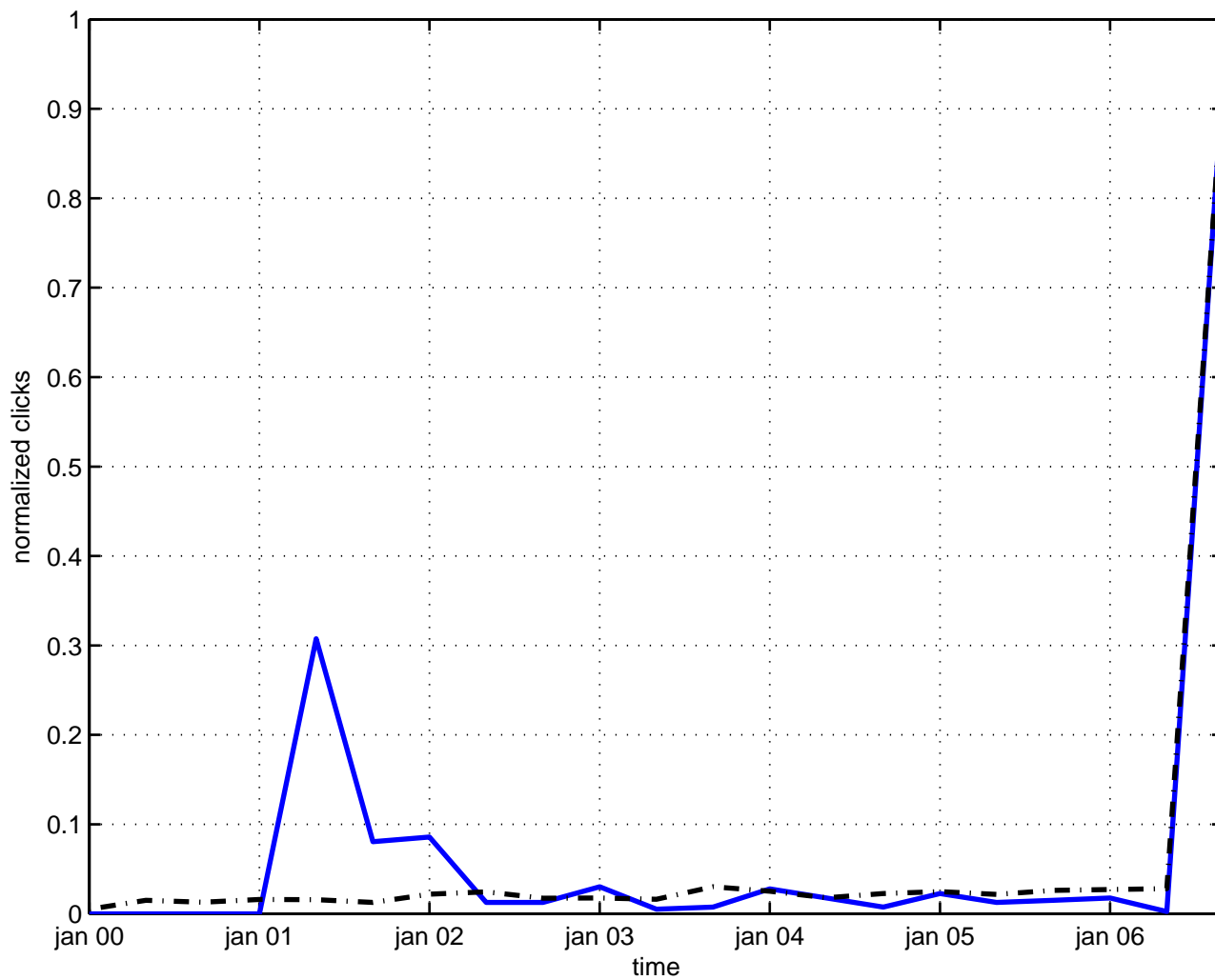
noncommutative surface
