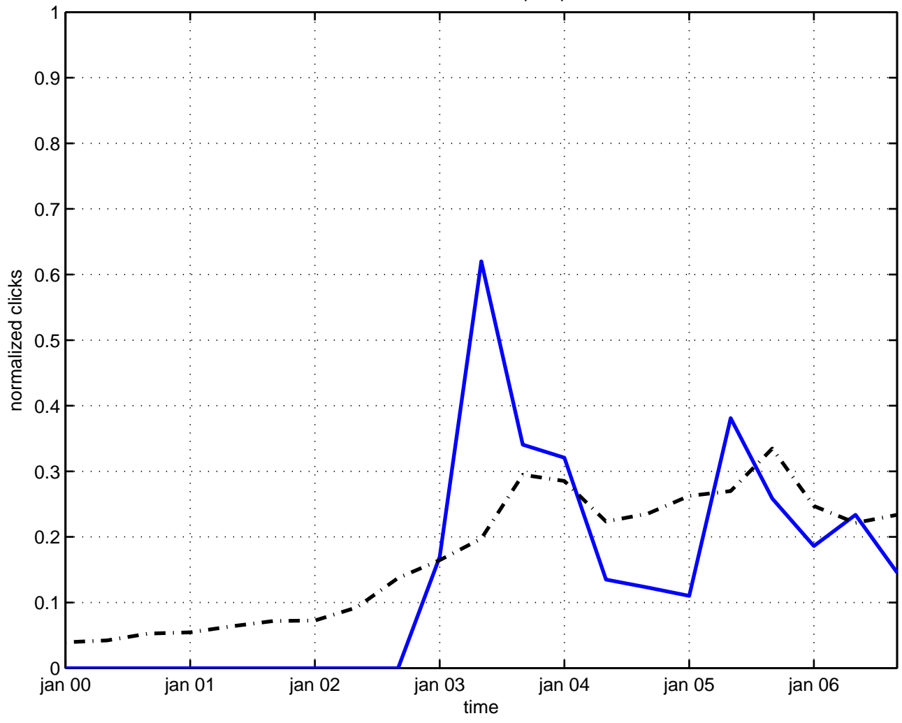
noncommutative superspace
