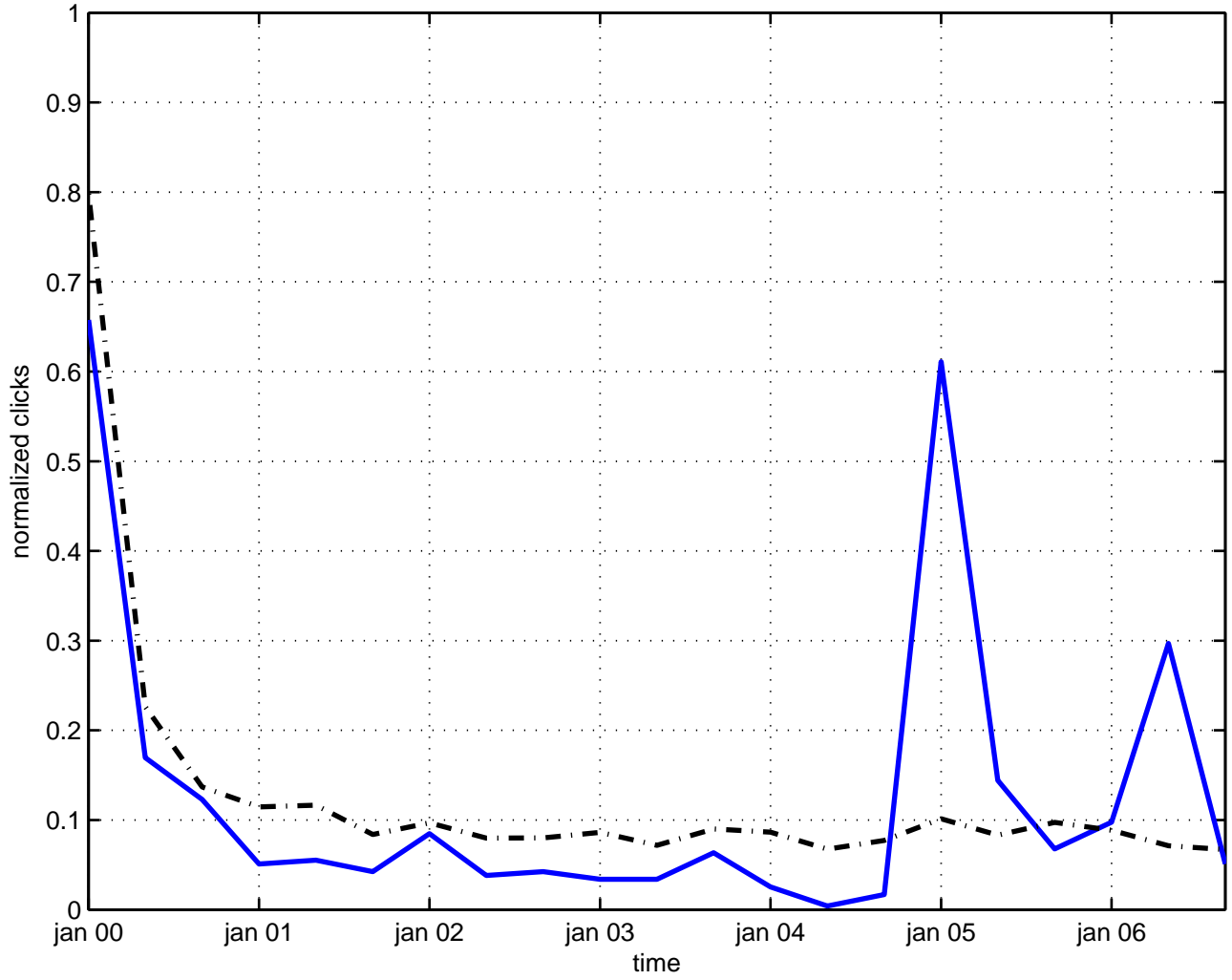
noncommutative string
