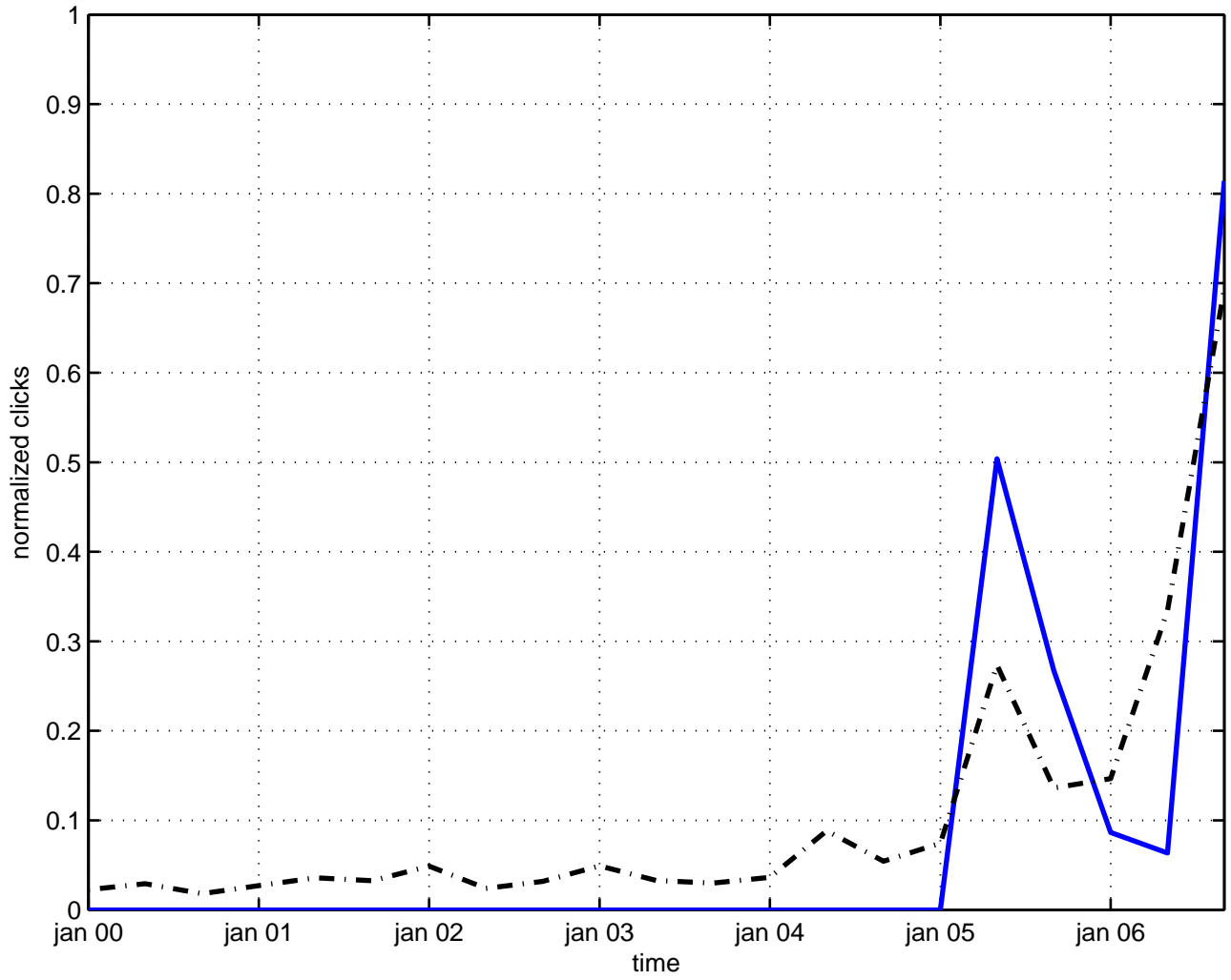
noncommutative standard model
