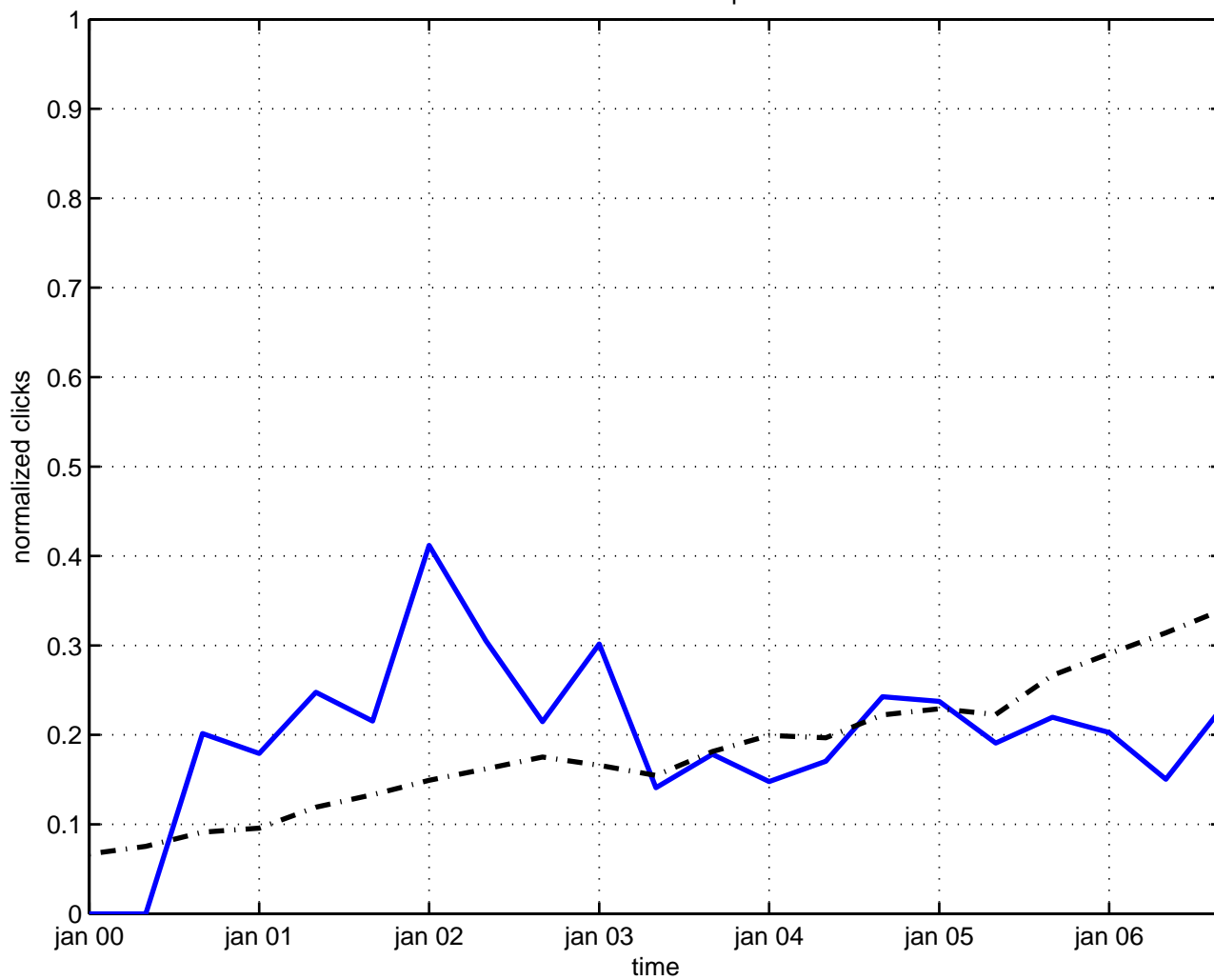
noncommutative space
